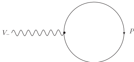
Figure 3. The only contribution to the effective action in unitary gauge.
