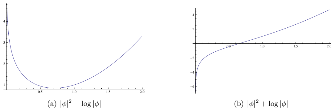
Figure 1. Plots of |\phi|^2 \mp \log |\phi| against |\phi| .
