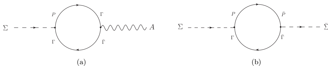
Figure 4. The remaining contributions to the effective action without gauge-fixing.
