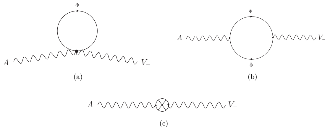
Figure 8. The three loops contributions to \langle AV_- \rangle coming loops of massless chiral fields.
