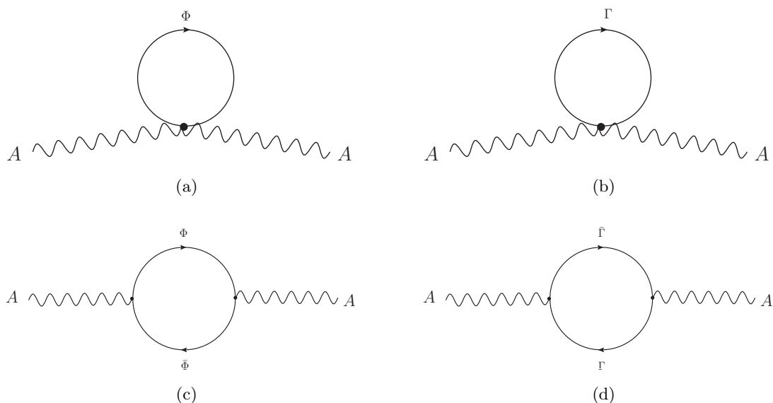
Figure 9. The diagrams contributing to \langle AA \rangle .
