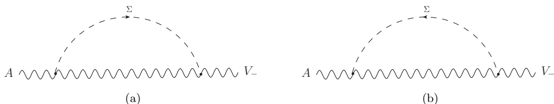
Figure 11. Novel contributions to \langle AV_- \rangle from \Sigma and gauge multiplet loops.
