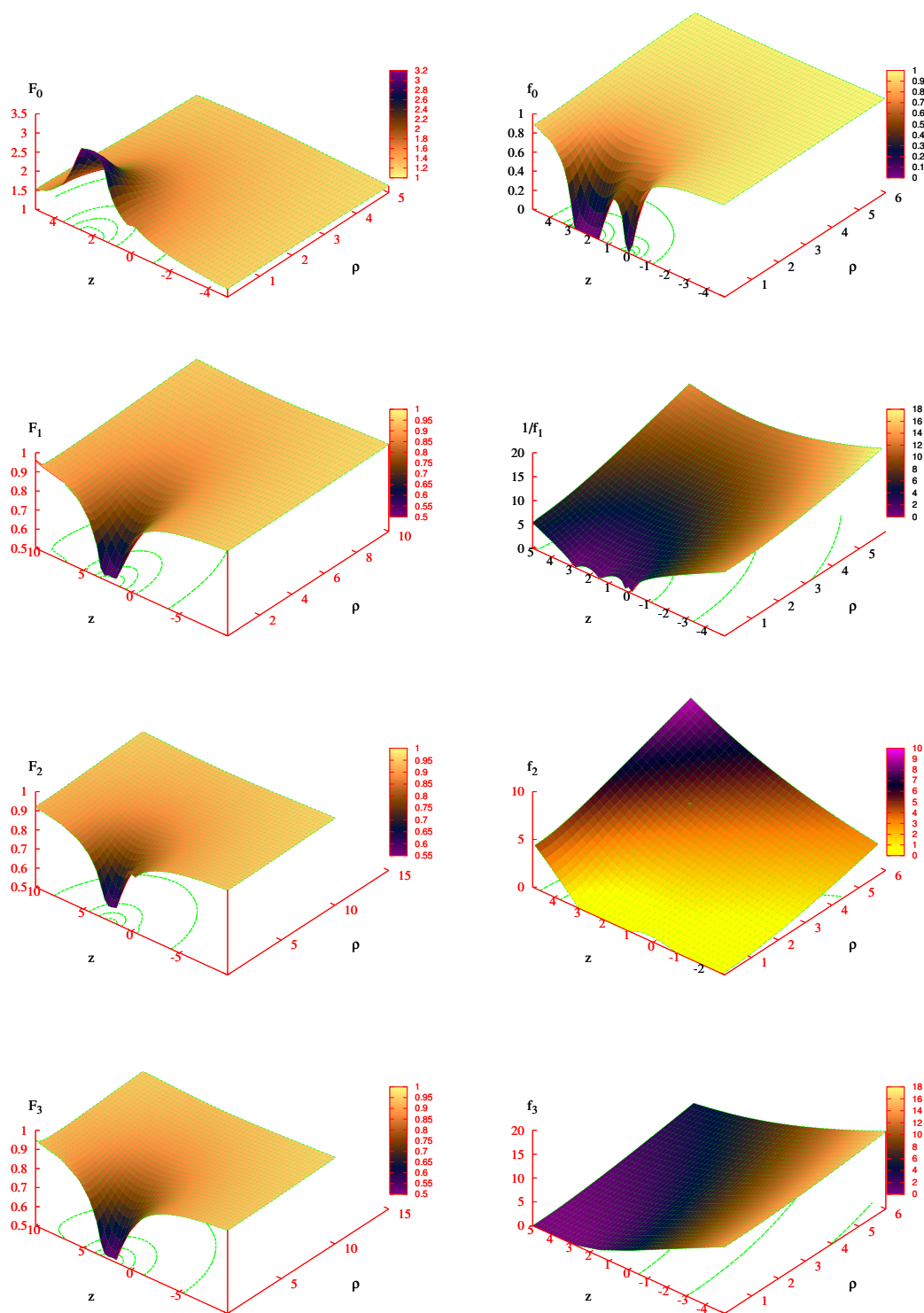
Figure 4. The profiles of the functions F_i used in the numerical calculations and of the metric functions f_i are shown for a typical d = 7 black Saturn-type solution with a = 0.14 , b = 1.5 , c = 2.8 .
