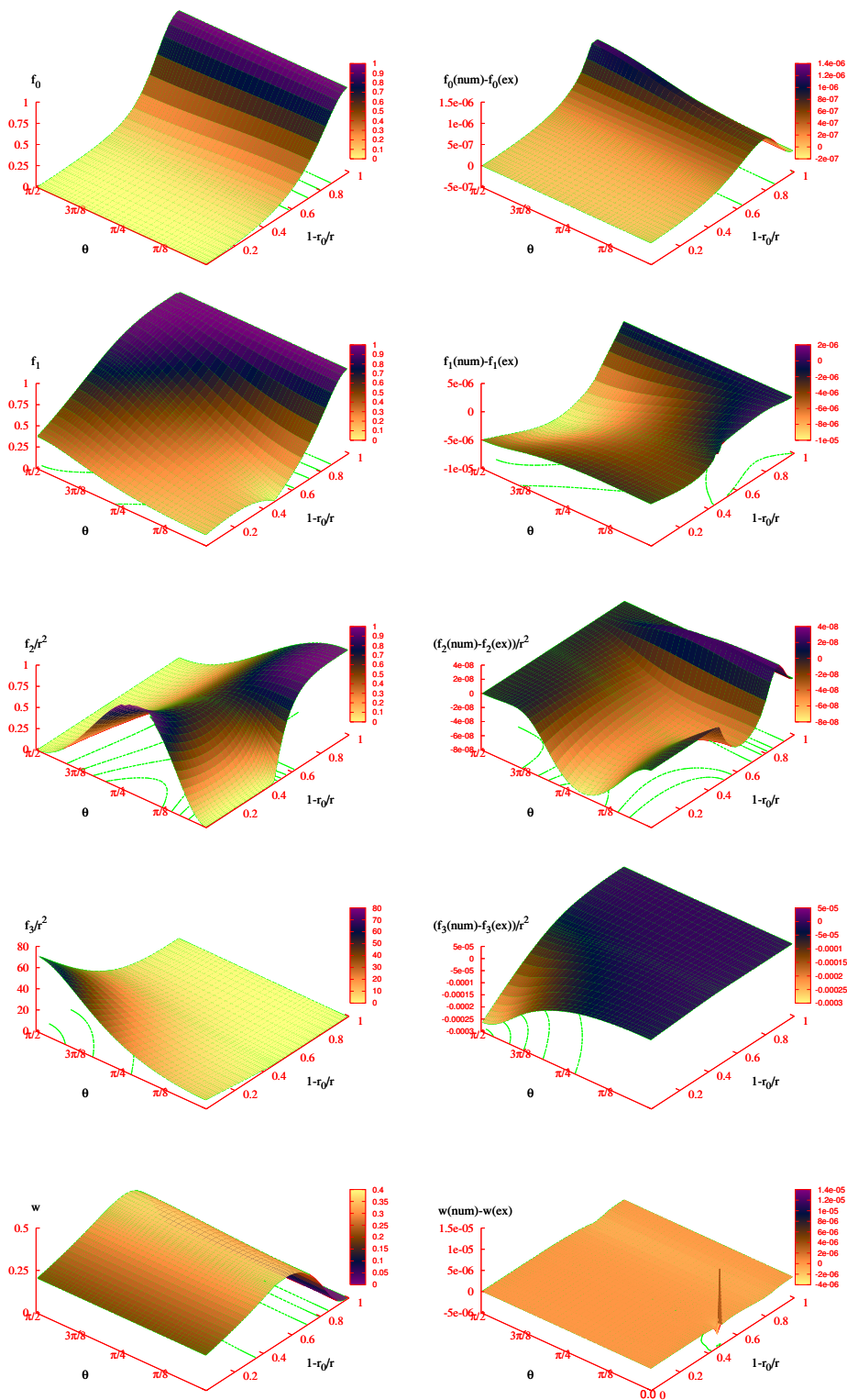
Figure 11. The metric functions f_i as given by (C.10) together with the difference between the exact solution and the numerical solution are shown for a typical d = 5 balanced black ring.
