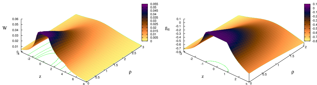
Figure 8. The metric function W (left) and g_{tt} = -f_0 + f_4 W^2 (right) are shown close to the horizon for a d = 7 rotating solution with S^2 \times S^3 event horizon topology. The input parameters here are a = 1 , b = 4 and \Omega_H = 0.05 . The contour line in the right panel indicates the ergo-region.
