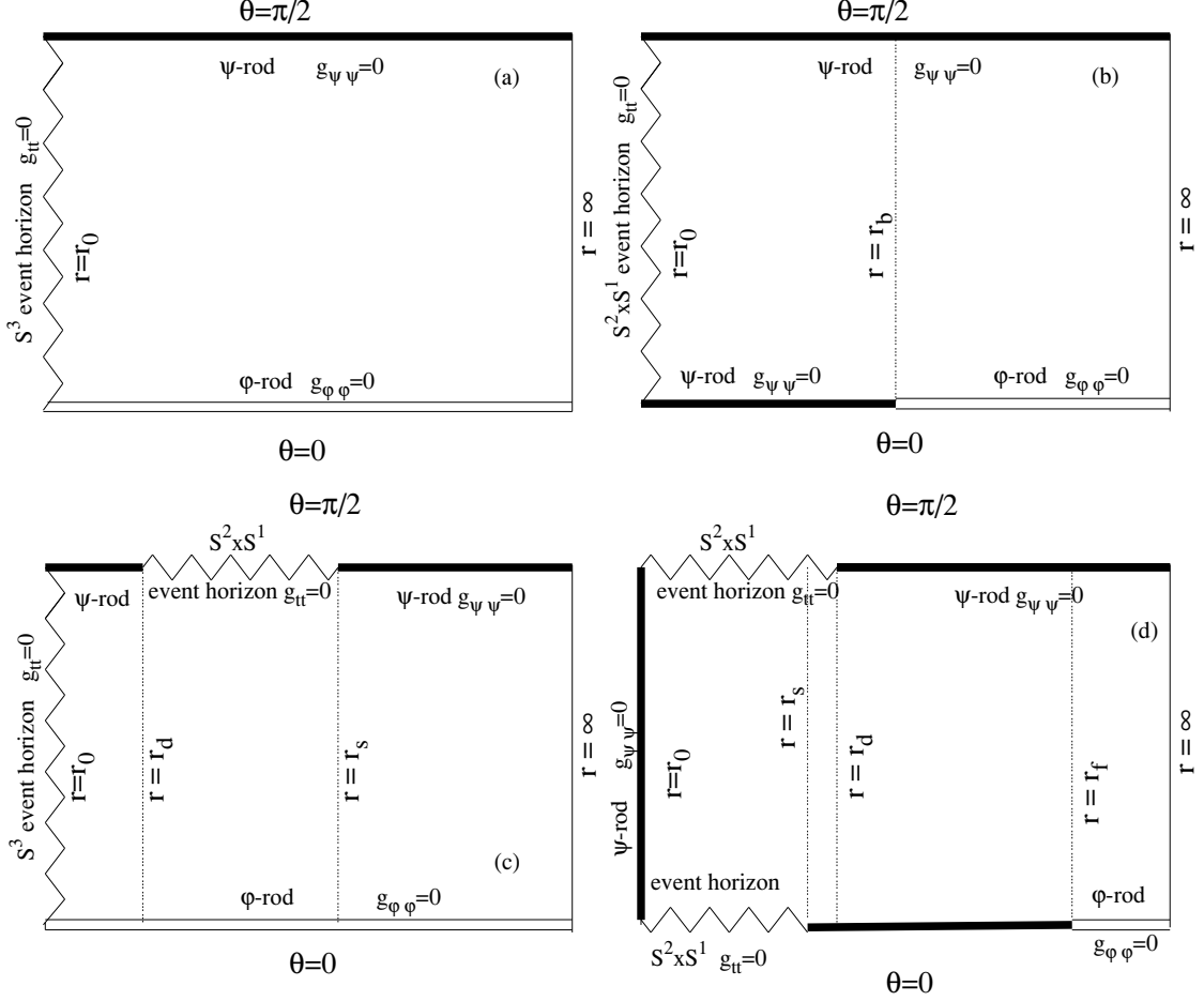
Figure 10. The domain of integration for the coordinate system (C.2) is shown for a Schwarzschild black hole, a static black ring, a black Saturn and a diring in d = 5 dimensions.
