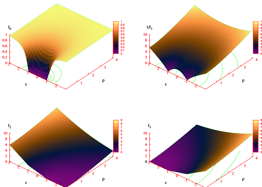
Figure 9. The profiles of the metric functions f_i for a d = 8 Schwarzschild-Tangherlini solution with a = 1 .
