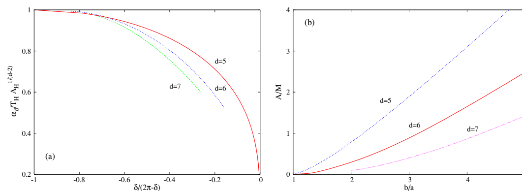
Figure 3. Features of generalized black ring solutions. (a): The scale free ratio T_H^{-1} A_H^{1/(d-2)} is shown as a function of the relative angular excess \bar{\delta} = \delta/(2\pi - \delta) . The parameter \alpha_d = (d - 3)2^{(5-2d)/(d-2)}\pi^{(3-d)/2(d-2)}\Gamma((d - 1)/2)^{1/(2-d)} has been chosen such that the point (-1, 1) on the plot corresponds to the Schwarzschild-Tangherlini black hole. (b): The scale free ratio \mathcal{A}/\mathcal{M} is shown as a function of the ratio between the two length scales b/a .
