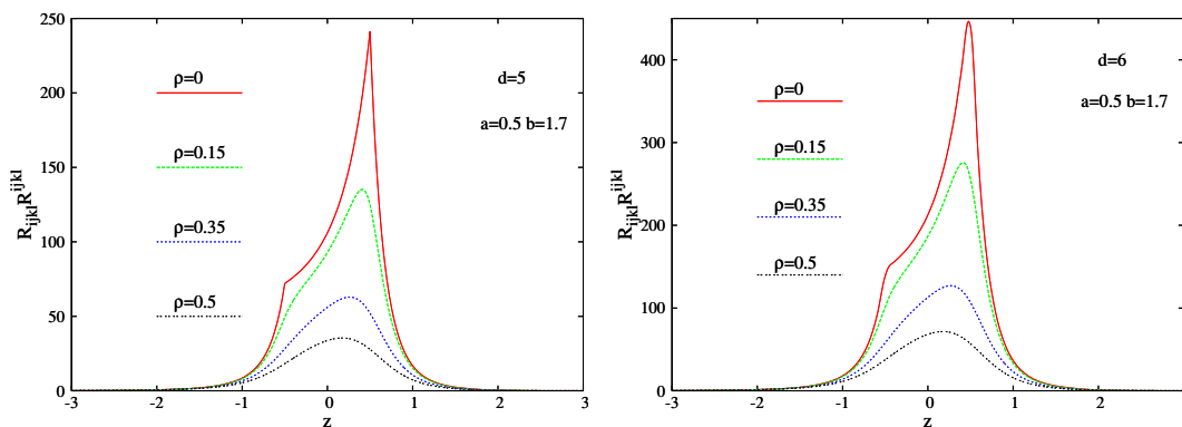
Figure 2. The Kretschmann scalar R_{ijkl}R^{ijkl} is plotted as a function of z for several values of \rho for d = 5, 6 black objects with S^2 \times S^{d-4} event horizon topology.
