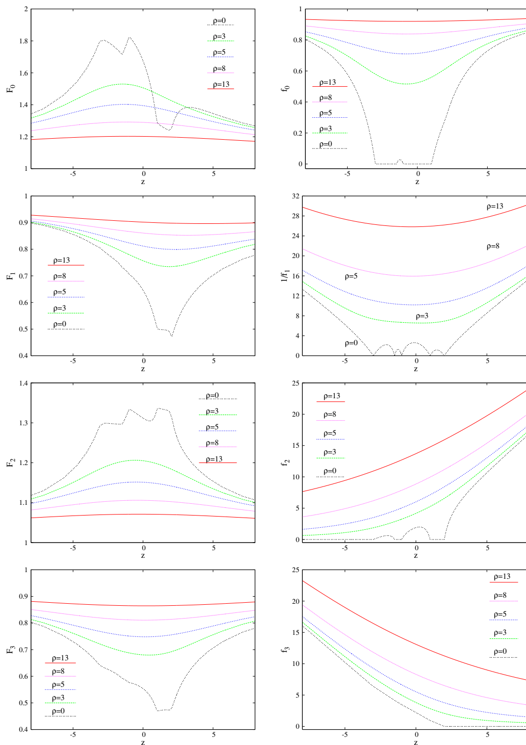
Figure 6. The profiles of the functions F_i used in the numerical calculations and of the metric functions f_i are shown for a typical d = 6 generalized black diring solution with a = 1, b = 2, c = 1.5, d = 3 .
