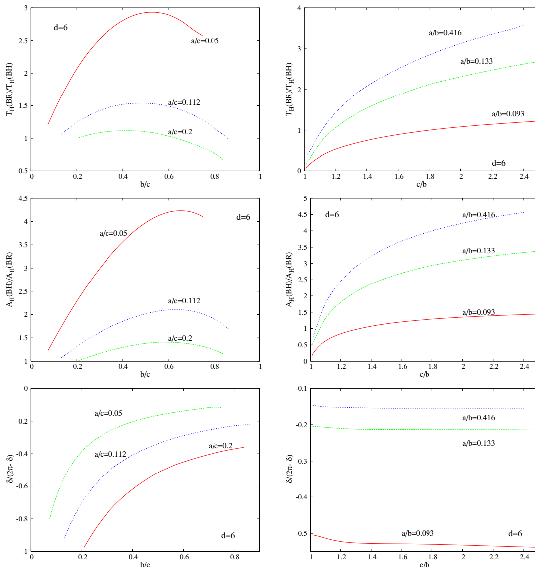
Figure 5. d = 6 generalized black Saturn solutions: a number of relevant dimensionless quantities are shown as a function of the ratio b/c for several fixed values of a/c (left) and for a varying ratio c/b for fixed a/b (right). In these plots the indices BR, BH stand for the objects with S^2 \times S^{d-4} and S^{d-2} horizon topology, respectively.
