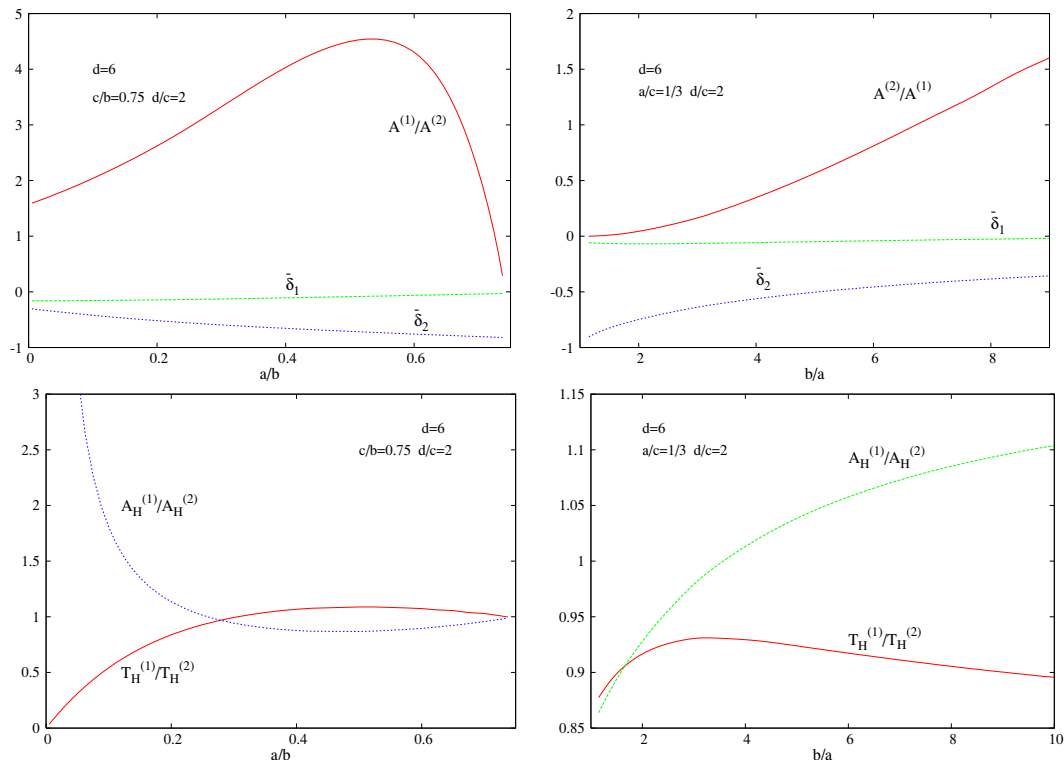
Figure 7. d = 6 generalized black diring solutions: a number of relevant quantities are shown as a function of the ratio a/b for several fixed values of c/b , d/c (left) and for a varying ratio b/a for fixed a/c , d/c (right). In these plots the indices 1, 2 stand for the objects with an event horizon at \rho = 0 , -d \leq z \leq -c and \rho = 0 , -a \leq z \leq a , respectively.
