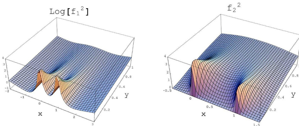
Figure 6. Metric factors f_1 and f_2 for a multi-pole Janus deformation. H is singular for x = 0, 1, \infty while A has poles in x = 0, -1, 1, 2 .
