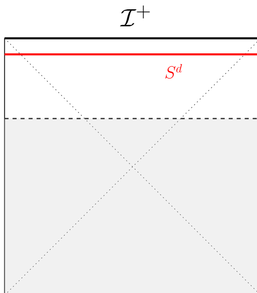
Figure 1. We are considering a late time slice (in red) with topology S^d in an asymptotically de Sitter spacetime. In the late time expansion, the Wheeler-DeWitt equation can be solved and, up to a universal phase factor, the space of solutions is the space of functionals that transform under \text{diff} \times \text{Weyl} in the same way as \text{CFT}_d partition functions.
