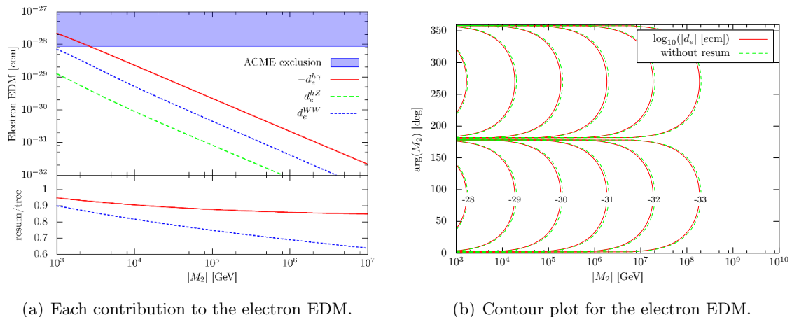
Figure 10. Results for the electron EDM. We take \tan\beta = 2 , \mu = 500 GeV, M_1 = M_2 and \tilde{m} = |M_2| . Left: each contribution to the electron EDM as a function of |M_2| . Red-solid, blue short-dashed, and green-dashed lines show the contribution of -d_e^{h\gamma} , d_e^{WW} , and -d_e^{hZ} , respectively. We set \phi_2 = \pi/2 . Blue-shaded region is excluded by the ACME experiment [92]. Lower panel illustrates the renormalization effects. Right: contour plot for the electron EDM. The red-solid and green-dashed lines represent the calculation with and without the resummation, respectively.
