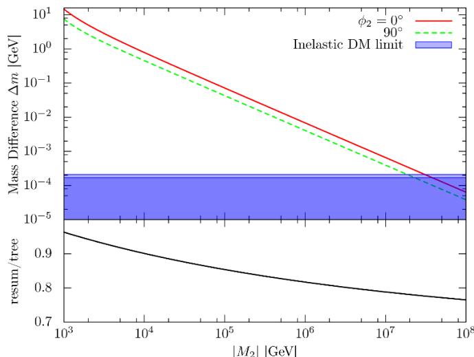
Figure 6. Mass difference \Delta m as functions of the Wino mass |M_2| in solid lines. Here, we take \tan \beta = 2 , \mu = 500 \text{ GeV} , M_1 = M_2 , and \tilde{m} = |M_2| . Red-solid and green-dashed lines show the \phi_2 \equiv \arg(M_2) = 0 and \pi/2 cases, respectively. Dark (light) shaded region illustrates the weakest (strongest) bound given in figure 5. The significance of the renormalization effects is shown in the lower graph.
