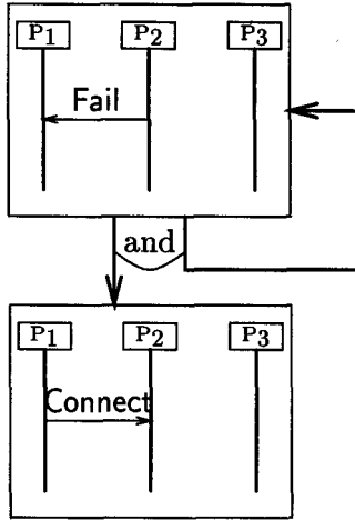
Fig. 2. A template MSC graph.
