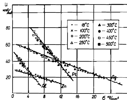
Fig. 6. Effective barrier U kcal/mol vs. tensile stress \sigma kg/mm 2 for polycrystalline metals.
