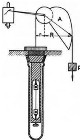
Fig. 1. Diagram of apparatus for long-duration studies of the lifetime of solids.
