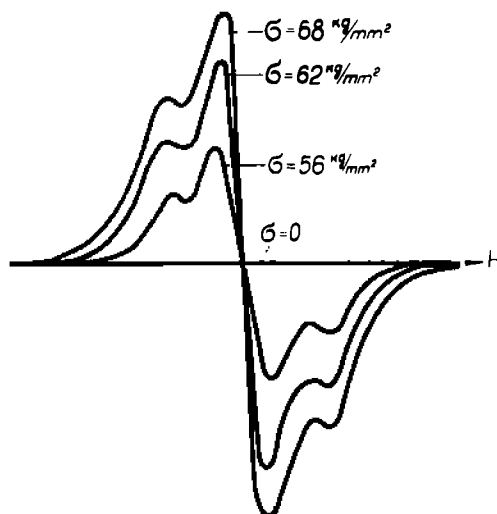
Fig. 9. EPR-spectrum of mechanically stressed capron fibres.
