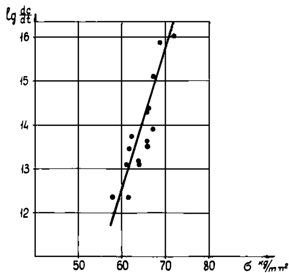
Fig. 10. Rate of formation of free radicals dc/dt vs. tensile stress.
