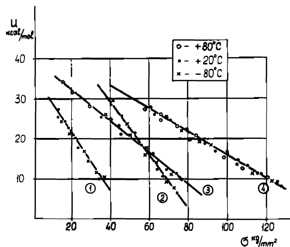
Fig. 7. Decrease of energy barrier U kcal/mol with tensile \sigma kg/mm 2 for polymers (fibres).
