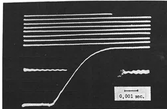
Fig. 4. Oscillographic recording of time to break for polycrystalline aluminum at stress of 6 \text{ kg/mm}^2 .
