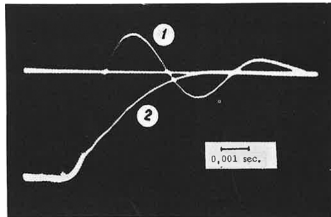
Fig. 3. Oscillogram of stress oscillations in a specimen in an impact test. 1. Without damper 2. With liquid damper.
