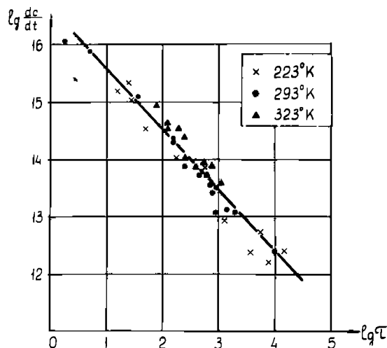
Fig. 11. Relation between the lifetime of capron fibres and rate of formation of free radicals at different stresses and temperatures.
