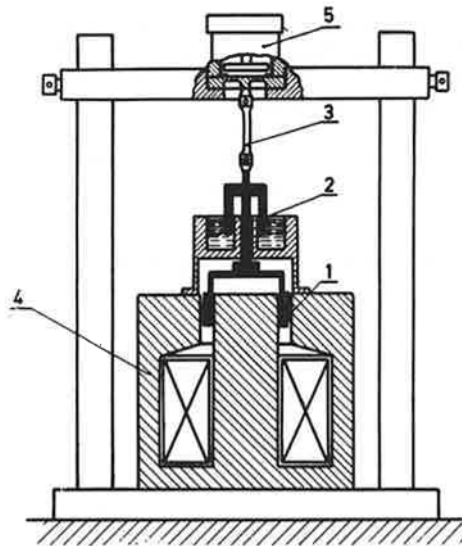
Fig. 2. Diagram of electromagnetic apparatus with a liquid damper for impact studies (Ref. 1.)
