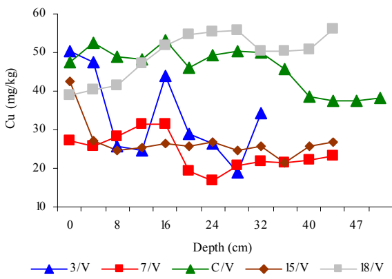
Fig. 4: Distribution of Cu in sediment cores
