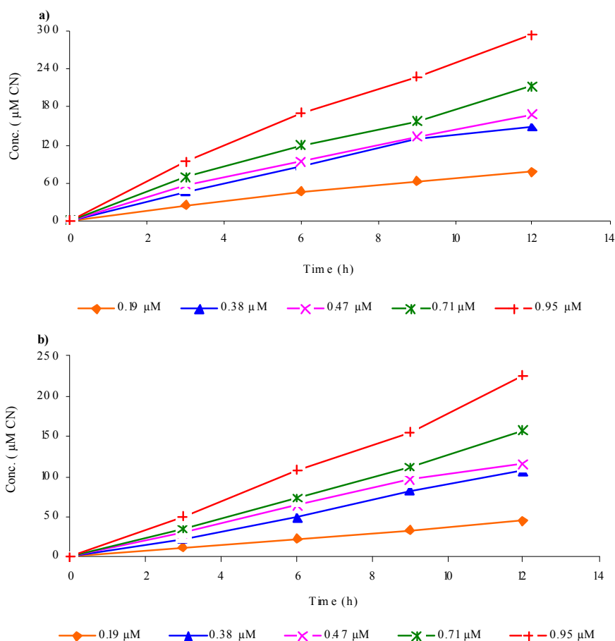
Fig. 3: Measured cyanide concentrations ( \mu\text{M CN} ) in aqueous solution at different initial concentrations, a) Ferri-cyanide dissolved in the 0.1 % NaOH solution; b) Ferri-cyanide dissolved in the deionized water. The values are the mean of two replicates for samples
