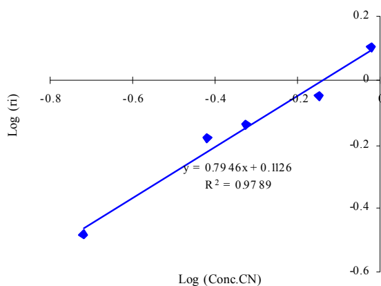
Fig. 4: Plot of \log(r_i) versus \log(\text{Conc.}_{\text{CN}}) in the treatment with ferri-cyanide. Reaction was performed at 20 °C with constant illumination intensity
