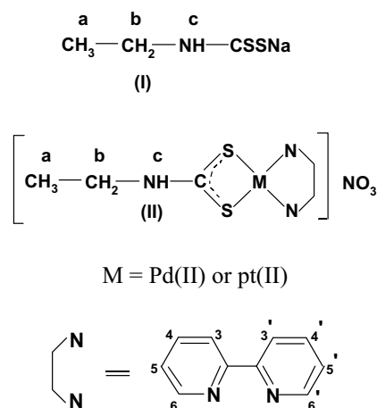
Fig. 1. Proposed structures and nmr numbering schemes of (I) Et-dtcNa, (II) [Pt(bpy)(Et-dtc)]NO 3 or [Pd(bpy)(Et-dtc)]NO 3
