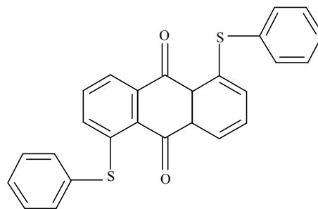
Bis-1,5-(thiophenyl)-9,10-anthraquinone (AQ1)
