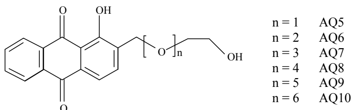
Scheme 2. Structure of the anthraquinone substituted podands AQ5-AQ10 [32].
