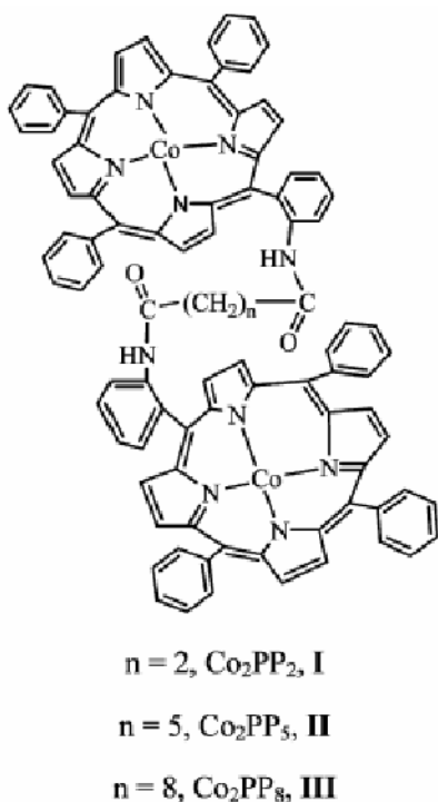
Scheme 4. The structure of dicobalt diporphyrin complexes.
