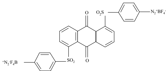
Bis-1,5-(benzenesulfonyl-4,4'-diazo)-9,10-AQ tetrafluoroborate (AQ4)
