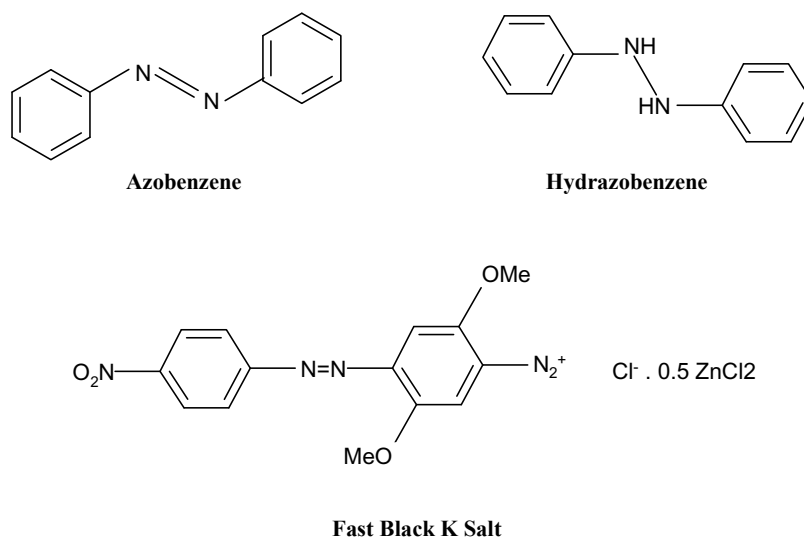
Scheme 3. The structure of azobenzene and its derivatives used for electrode modification.
