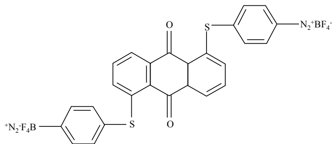
Bis-1,5-(Thiophenyl-4,4'-diazo)-9,10-AQ tetrafluoroborate (AQ3)
