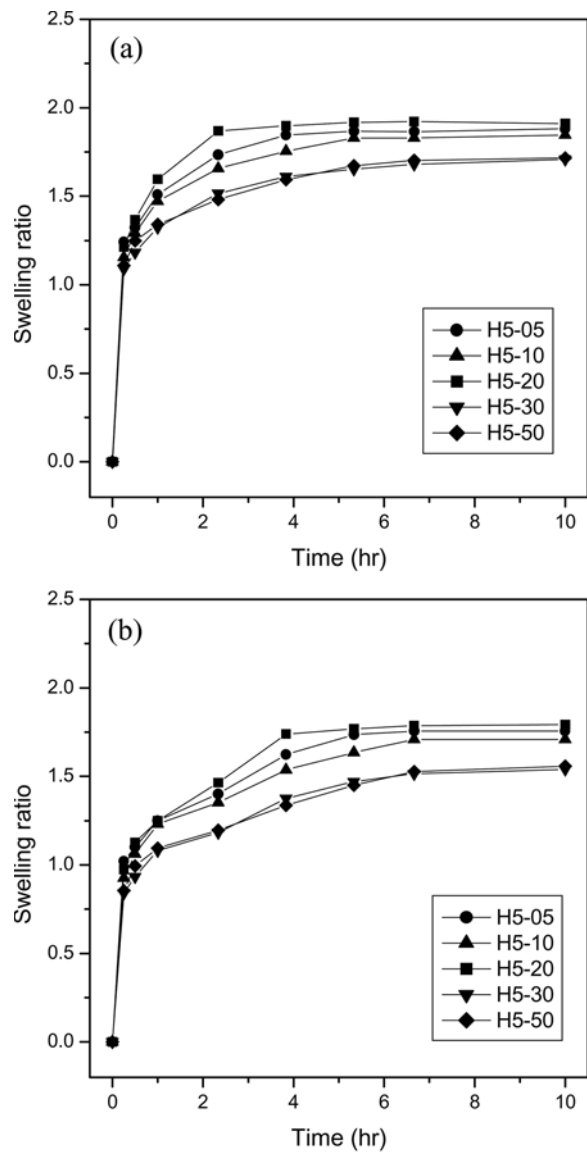
Figure 4. Swelling kinetics of alginate-g-NIPAAm hydrogels in deionized water (pH = 5.4). (a) 25 °C and (b) 37 °C.
