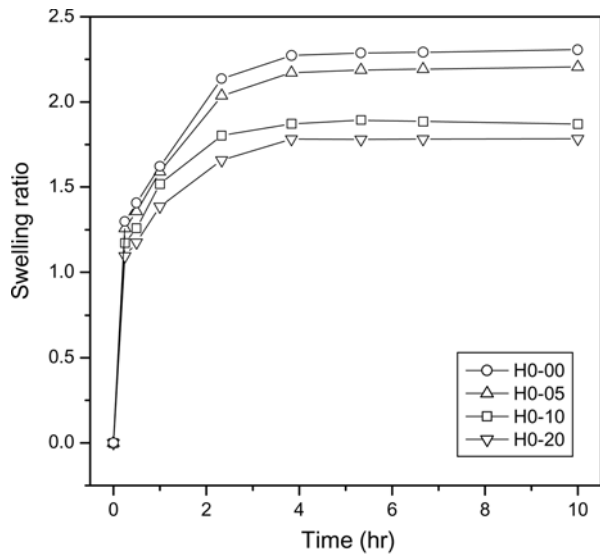
Figure 3. Swelling kinetics of the alginate films which were treated at various irradiation doses in the deionized water (25 °C and pH = 5.4)
