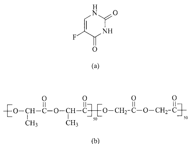
Figure 1. Chemical structures of (a) 5-FU and (b) PLGA (50/50).
