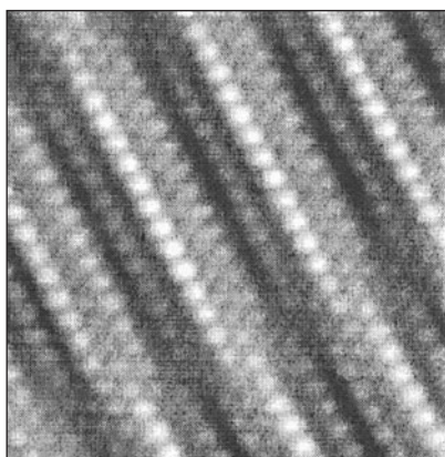
Figure 4 High resolution STM image of the reconstructed Au (100)-(1x5) surface (size 5.3 x 5.3 nm 2 ). (62)
