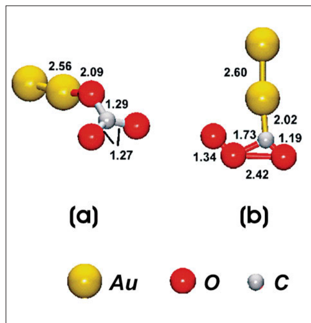
Figure 8 Two forms of Au 2 CO 3 relevant to CO 2 production. a) digold carbonate and b) digold-peroxyformate with calculated bond lengths indicated. (185)
