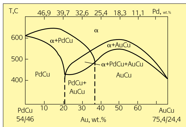
Figure 2 Pseudo-binary phase diagram of the \text{PdCu-AuCu} system [4]
