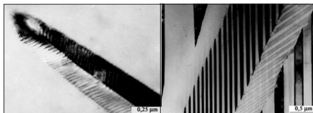
Figure 4a Formation of a microstructure in an equiatomic CuAu alloy during ordering [6]: a - initial stages of formation of a lamellar structure;
