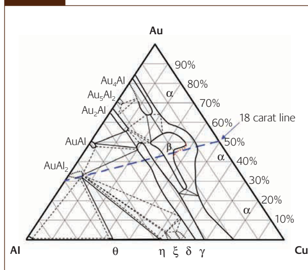
Proposed isothermal section through Al-Au-Cu system at 500°C (reproduced from Levey and Cortie[3]) in atomic percent. The dashed blue line shows the position of the 18 carat isopleth. The dotted red line designates that there is some uncertainty in the position of the \beta phase boundary in the indicated region
