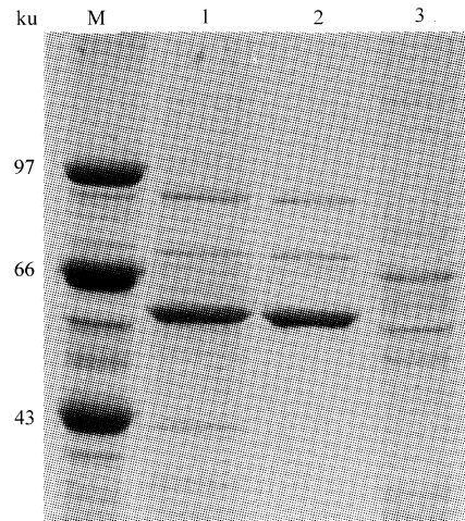
Fig. 2. Coomassie Brilliant Blue stained SDS-polyacrylamide gel electrophoresis of rAAV-GFP at various stages of purification. Each stock was mixed with an equal volume of 2 \times loading buffer and incubated in boiling water for 3 min before loading. 10 \mu\text{L} sample was loaded in each lane. The start material was shown in lane 3. The crudely purified stock of rAAV-GFP is shown in lane 1, and the purified rAAV-GFP is shown in lane 2. M, Standard proteins whose molecular weights are indicated on the left.
