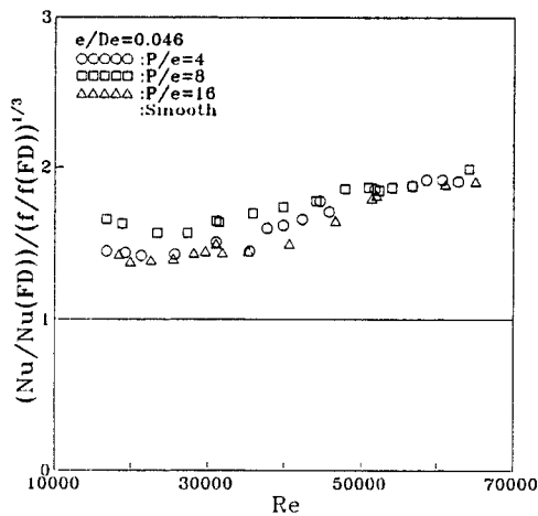
Fig. 8 Efficiency index
