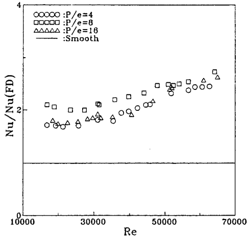
Fig. 7 Normalized Nusselt number
