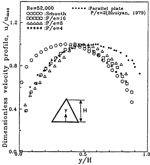
Fig. 2 Velocity profiles
