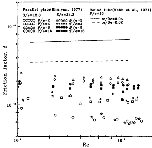
Fig. 4 Friction factors for similarly configured channels(Bhyuyan, 1977; Webb et al., 1971)
