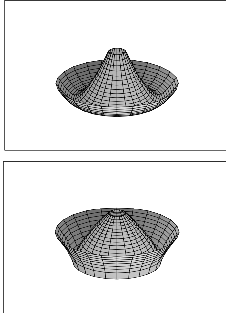
FIG. 2. Surfaces containing cycle spirals of Lipschitz and Hölder types
