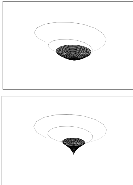
FIG. 1. Focus spirals of Lipschitz and Hölder types
