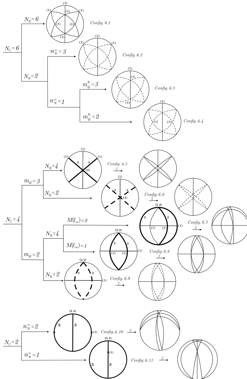
Diagram 1 ( M_{IL} = 6 )
