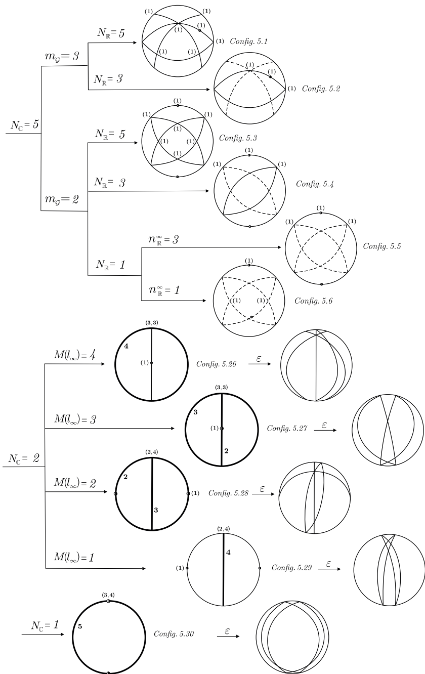
Diagram 2 ( M_{\text{IL}} = 5 )
