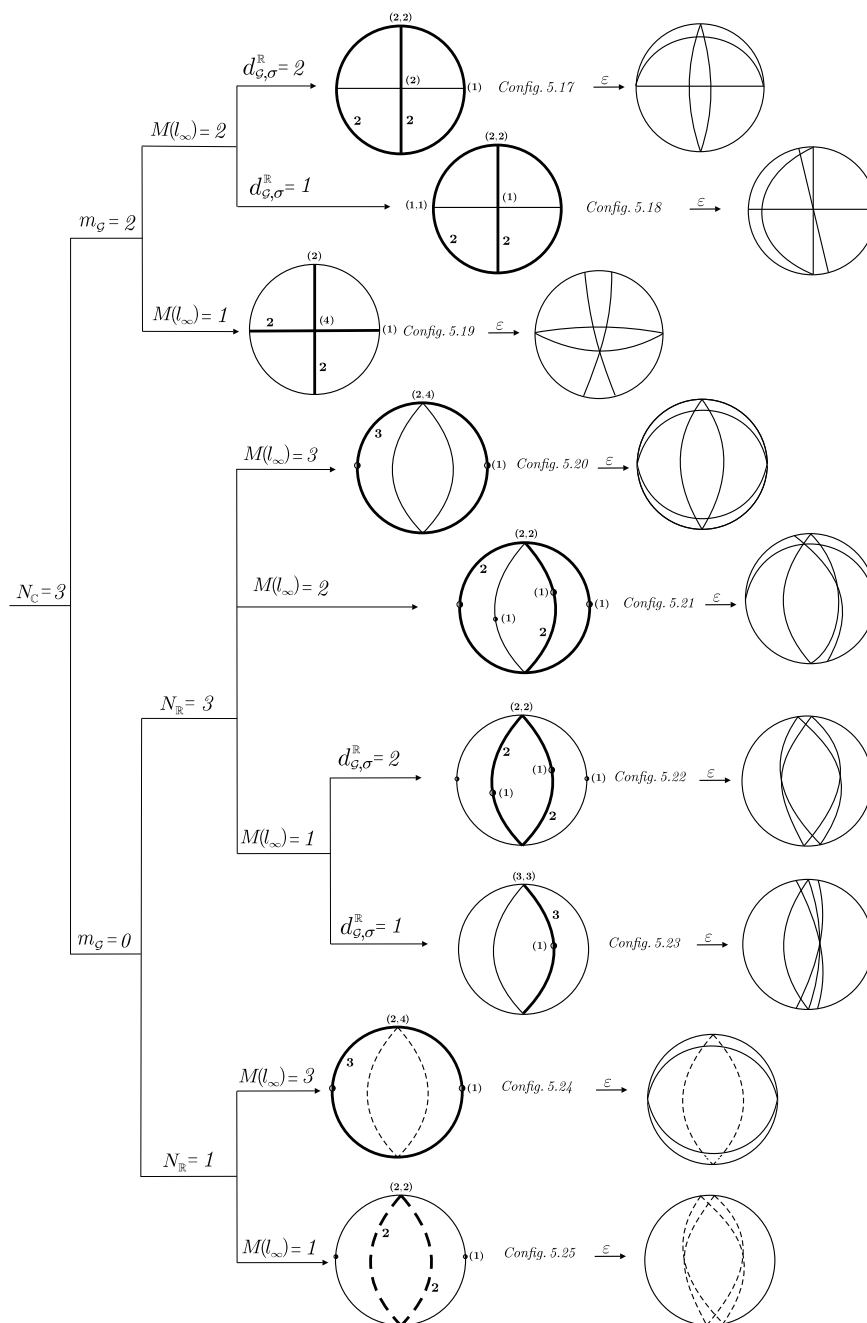
Diagram 2 ( M_{\text{II}} = 5 ) (continued)
