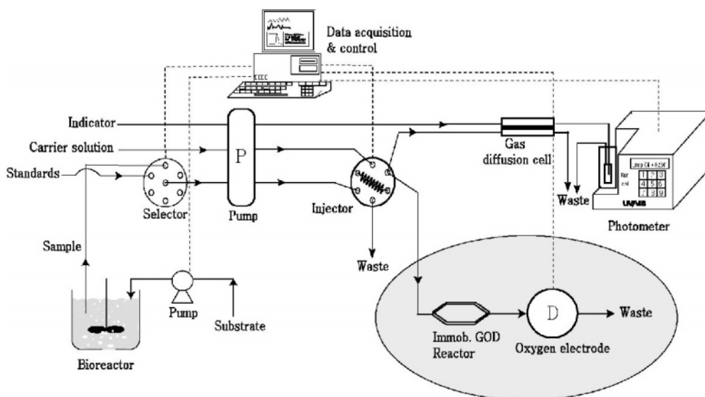
Fig. 1. Set-up of Glucose-FIA and Ammonia-FIA
