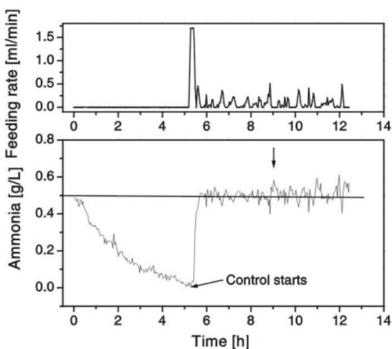
Fig. 10. Time course of ammonia concentration and feeding rate in a CSTR controlled by a NN-based controller (set point : 0.5 g/L). Solid line represents on-line FIA data.
