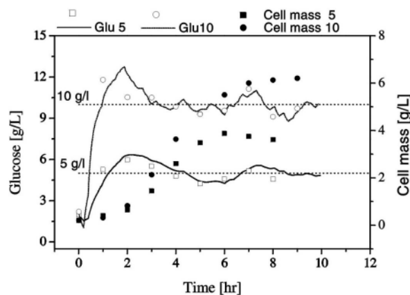
Fig. 2. Time courses of glucose and cell mass production in the cultivation of S. cerevisiae controlled to 5 g/L and 10 g/L by on-off controllers. Symbols ( \square , \circ , \blacksquare , \bullet ) represent off-line data for glucose and cell mass, while lines represent on-line FIA data (Analysis frequency of the glucose-FIA: 24 1/hr).
