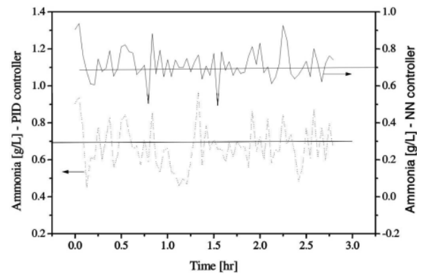
Fig. 8. Experimental comparison of a 3-2-1 NN-based controller with a PID controller for the control of ammonia concentration to 0.7 g/L (5% measurement error, 150 training cycles). Solid line represents on-line FIA data controlled by the NN controller, while dotted line represents on-line FIA data controlled by the PID controller.
