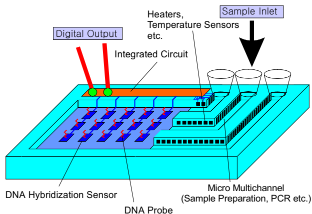
Fig. 6. Laboratory-on-a-chip.
