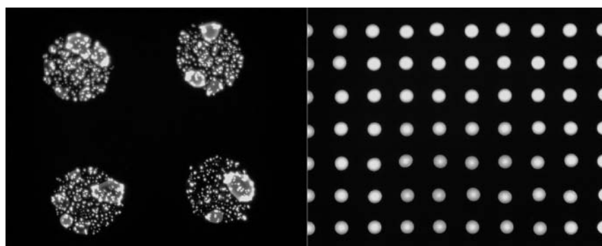
Fig. 6. Fluorescence image of DNA hybridized array.
