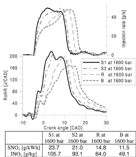
Fig. 9 Effect of rate shaping at a constant maximum injection pressure of 1600 bar and SOI -8 CAD ATDC
