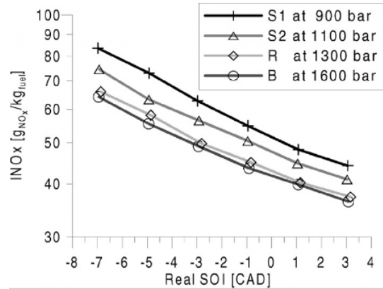
Fig. 10 INO x dependency for constant injection duration vs SOI
