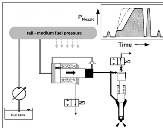
Fig. 1 Amplifier piston common rail system
