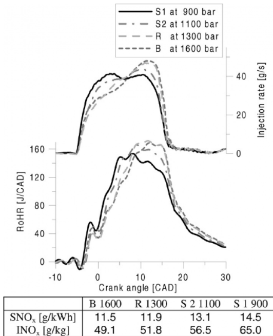
Fig. 8 Effect of rate shaping at constant injection duration on combustion and emissions for SOI -8 CAD ATDC
