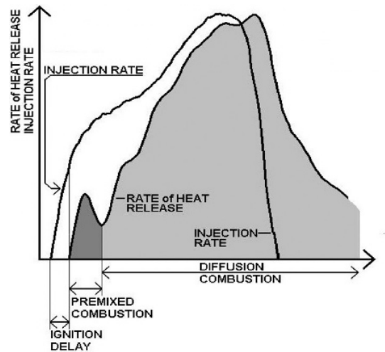
Fig. 5 Ignition delay, premixed combustion (Boot at 1600 bar)
