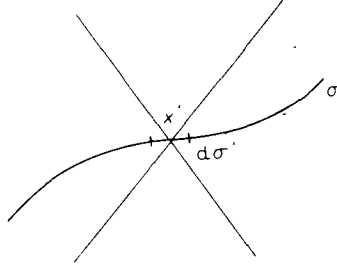
Fig. 4. — Space-time picture of a covariantly defined position measurement performed upon a Klein-Gordon particle: does the particle pass or not an arbitrary element d\sigma^a at x^2 on a spacelike surface \sigma ? The corresponding eigenfunction is the Jordan-Pauli propagator with apex at x , nonzero inside both the future and the past light-cone. Thus the wave collapse affects symmetrically the future and the past .
