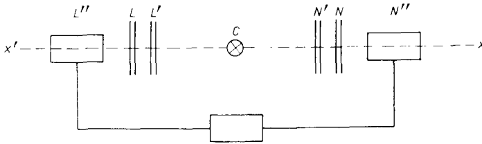
Fig. 1. — Photon polarization correlation experiments. C , atomic cascade; L' , N' , monochromatic filters; L and N , linear polarizers with adjustable angles A , B ( A - B = \alpha ); L'' , N'' , coincident photodetectors.
