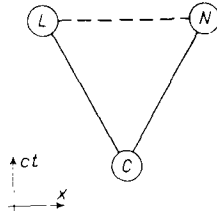
Fig. 2. — Space-time diagram of the Einstein paradox: the die is cast not at the severance point-instant C , but later, at L and N , where and when the measurements are performed. Thus the correlation between L and N is tied through C , in their common past, via the Feynman-style zigzag made of the timelike vectors CL and CN .
