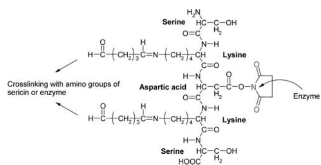
Figure 1. Schematic representation of reactions of sericin fixation and enzyme immobilization. The names of amino acids are in bold characters.
