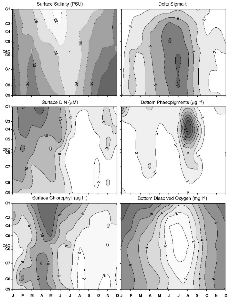
Fig. 4. Water column parameters along transect C (location in Fig. 2) from station C1 inshore at 5 m to C9 offshore at 30 m, January–December 1985–2001. Modified from Rabalais et al. (2002c).
