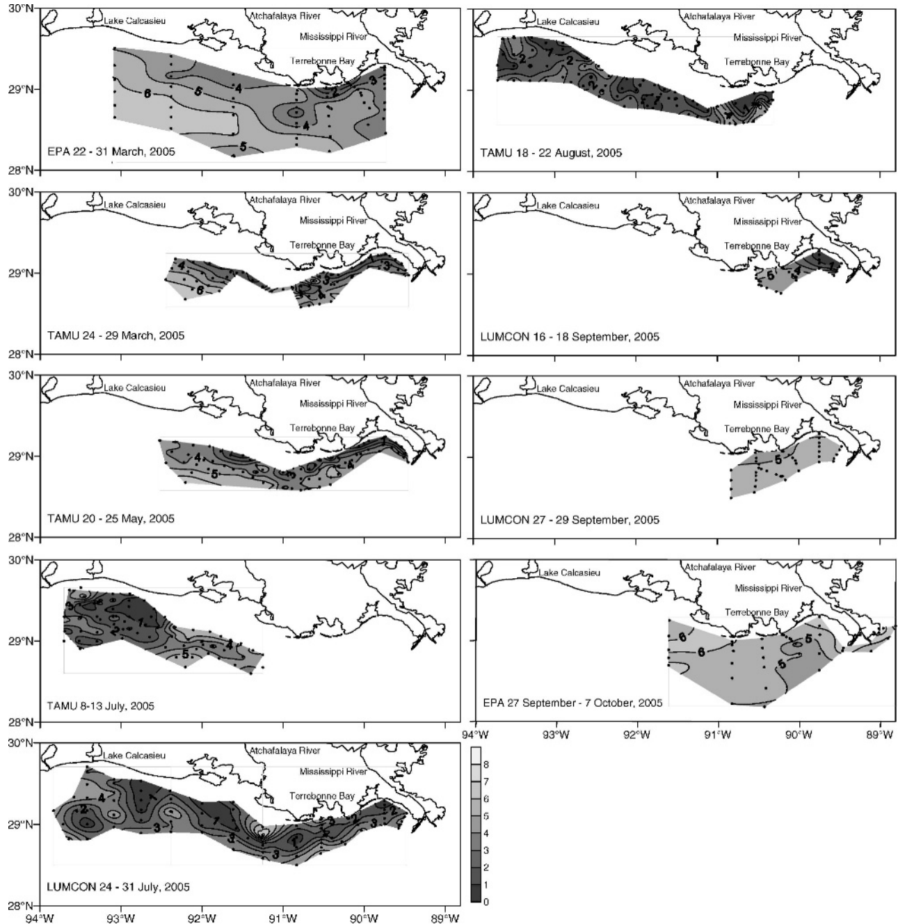
Fig. 3. Dissolved oxygen contours ( \text{mg l}^{-1} ) for cruises in 2005. Isoleths were contoured in Surfer 8 using ordinary point Kriging. An anisotropy ratio of 2 was applied to account for the general east-west direction of the bathymetric contours. Unpublished data of N. N. Rabalais, Louisiana Universities Marine Consortium (LUMCON), M. C. Murrell, U. S. Environmental Protection Agency, Gulf Breeze, Florida (EPA), and S. DiMarco (TAMU) and their colleagues in hypoxia research. Data source and periods are identified in each panel.
