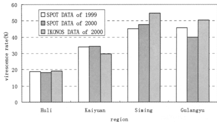
Figure 4 Comparison of vegetation investigation data by remote sensing in the years 1995 and 2000
