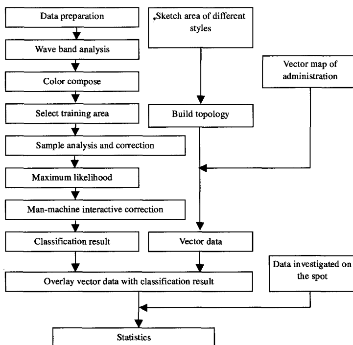
Figure 3 Classification process for very high resolution remote sensing image
