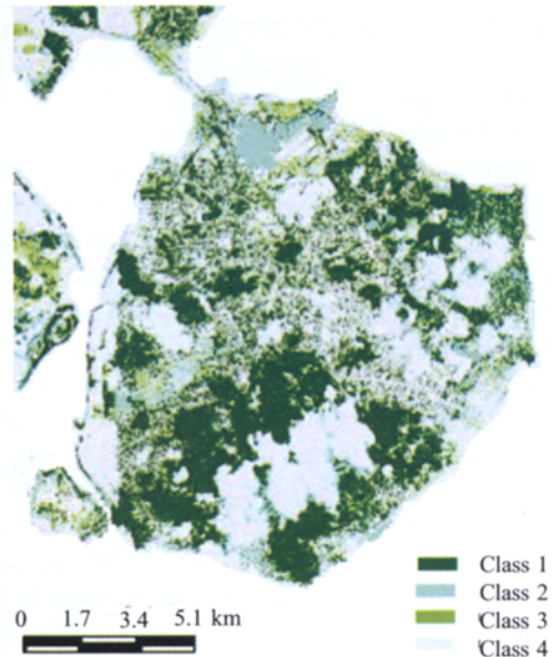
Figure 2 Maximum likelihood classification in east of Kaiyuan District and the mountain area in Siming District of Xiamen
