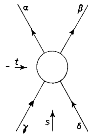
Fig. 1. - Schematic diagram of \pi\pi scattering, with isospin indices \alpha, \beta, \gamma, \delta .
