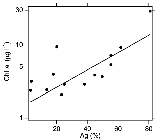
Fig. 4. Median chl a at all sites as a function of percent of watershed that is comprised of agricultural land use (Ag). The line is a linear curve fit through the points. The Spearman correlation coefficient between the values is r_s = 0.74 ( p = 0.014 ).
