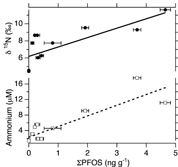
Fig. 7. Median \delta^{15}\text{N} and ammonium concentrations in water as a function of \Sigma\text{PFOS} concentrations in sediments. Error bars represent 95% confidence intervals for the triplicate \Sigma\text{PFOS} measurements taken from each sediment sample. The lines show the best linear fit between the data.
