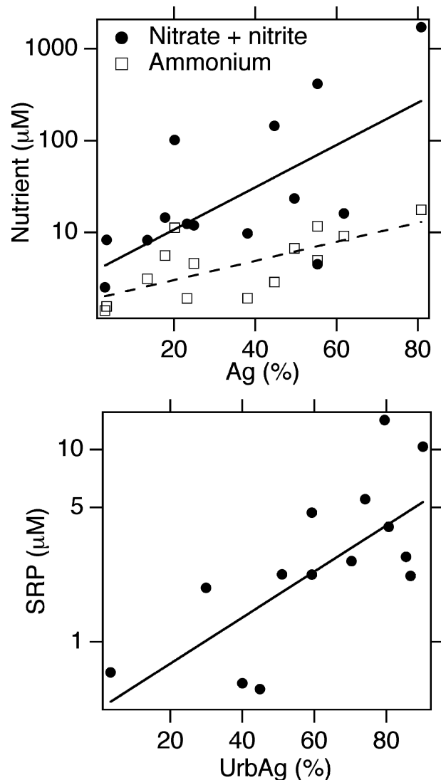
Fig. 3. Median concentrations of nitrate + nitrite and ammonium measured at all the sites as a function of percent of watershed that is comprised of agricultural land use (Ag). The lines represent a linear curve fit through the points. The Spearman correlation coefficients between the values are r_s = 0.59 ( p = 0.025 ) for nitrate + nitrite and r_s = 0.69 ( p = 0.0067 ) for ammonium. The median concentrations of soluble reactive phosphate (SRP) measured at all the sites as a function of percent of watershed that is comprised of urban and agricultural land use (UrbAg). The line represents a linear curve fit through the points. The Spearman correlation coefficient between the values is r_s = 0.69 ( p = 0.0067 ).
