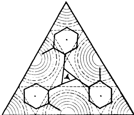
Fig. 5. - (220) structure factor graph, showing the position assumed by the macromolecule (contours are drawn at regular intervals: — positive lines; - - - - zero lines; - - - - negative lines).
