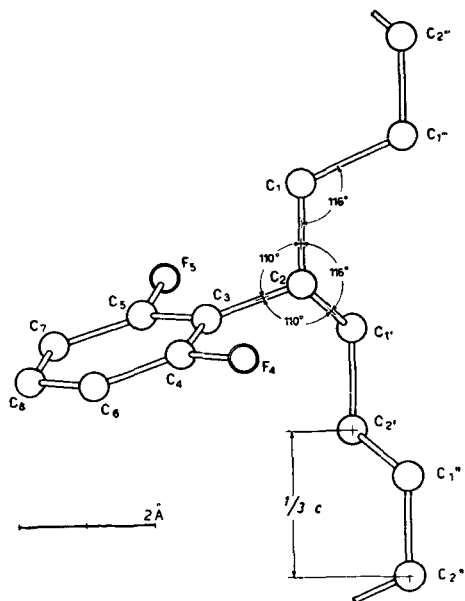
Fig. 4. - Conformation of the independent structural unit of poly-ortho-fluorostyrene ( C-C = 1.54 \text{ \AA} , (C-C)_{\text{ortho}} = 1.40 \text{ \AA} , C-F = 1.35 \text{ \AA} , CCF = 120^\circ ).
