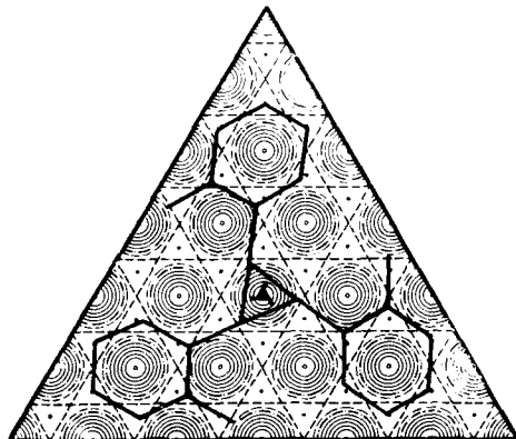
Fig. 6. — (660) structure factor graph.
