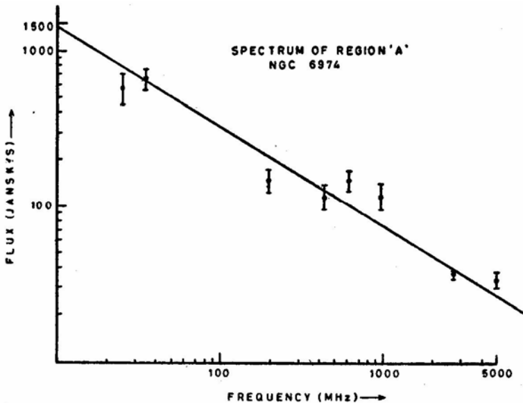
Figure 5. Spectrum of Region A (NGC 6974).
