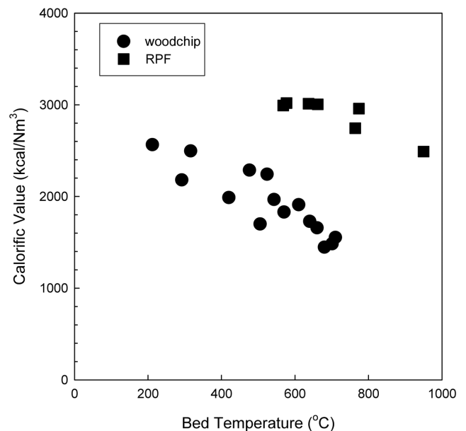
Fig. 5. Effect of bed temperature on calorific value of the produced gas.
