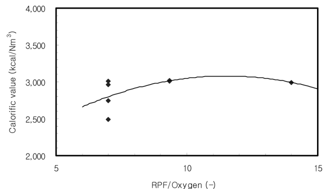
Fig. 6. Effect of RPF/O 2 ratio on calorific value of the produced gas.
