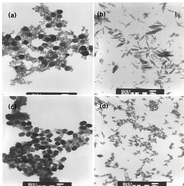
Fig. 6. Transmission electron micrographs (TEM) of \alpha -Fe 2 O 3 particles obtained by aging 0.02 M FeCl 3 aqueous solution containing Pionin NDA and Pionin CLS at 100 °C for 12 hrs. Pionin NDA (a) 0.1 g/l, (b) 0.5 g/l, Pionin CLS (c) 0.1 g/l, (d) 0.5 g/l.
