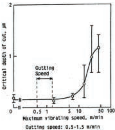
Figure 13. Effect of tool vibration speed on critical depth of cut (Moriwaki et al 1992).
