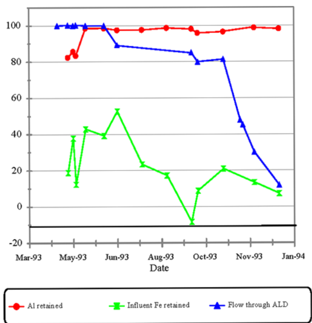
Figure 3. Flow of water through ALD and percent of influent aluminum and iron retained in the ALD at Jennings.
