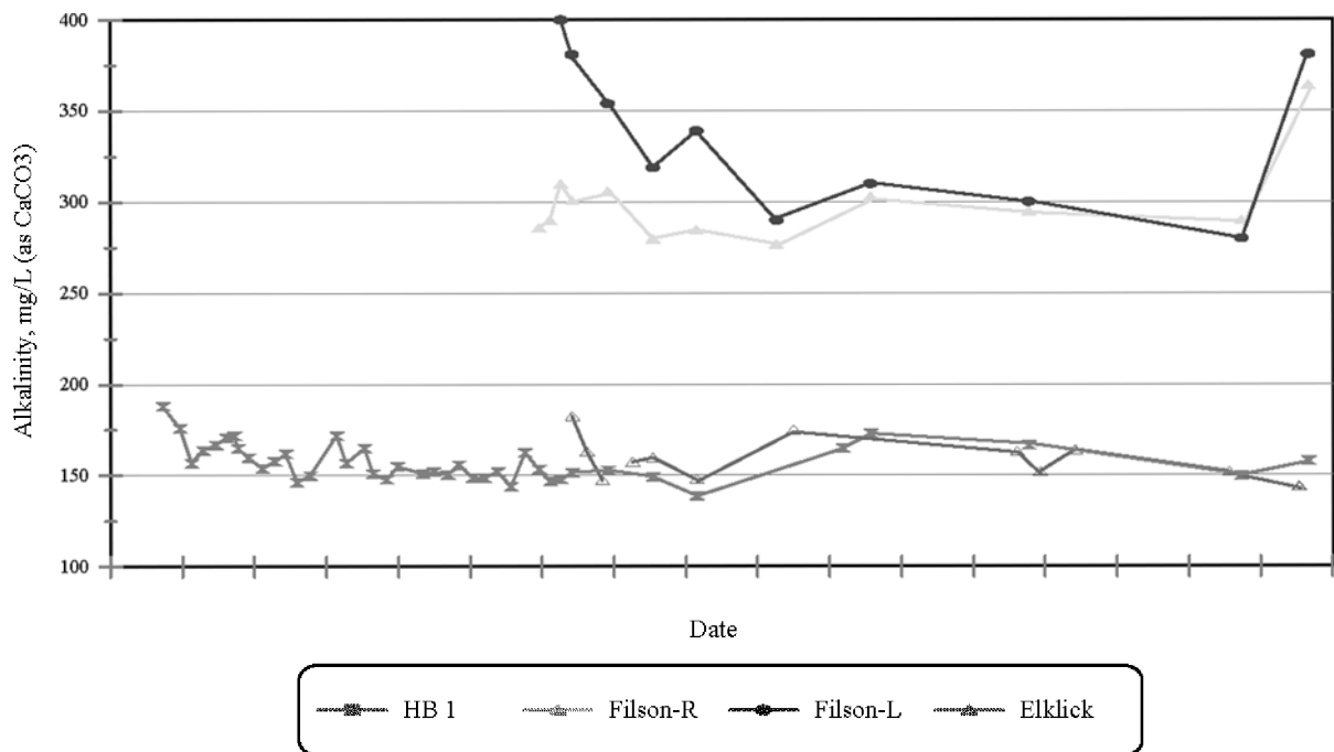
Figure 2. Effluent alkalinity concentrations of selected ALDs.
