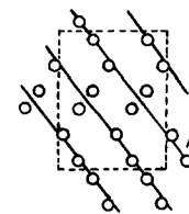
PROJECTION OF CEMENTITE IN THE [100] DIRECTION
