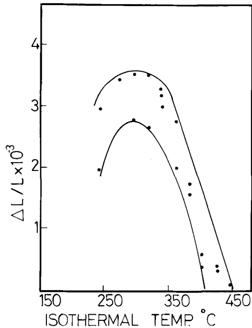
Fig. 3—Curve of dL versus isothermal transformation temperature showing temperature dependency of the 'incomplete reaction' phenomenon.
