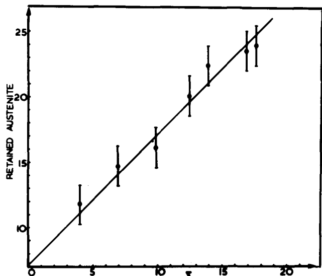
Fig. 8—The variation of upper bainitic retained austenite with the parameter \Sigma = 17.5P_{022\alpha} + (124,300/d^3) .
