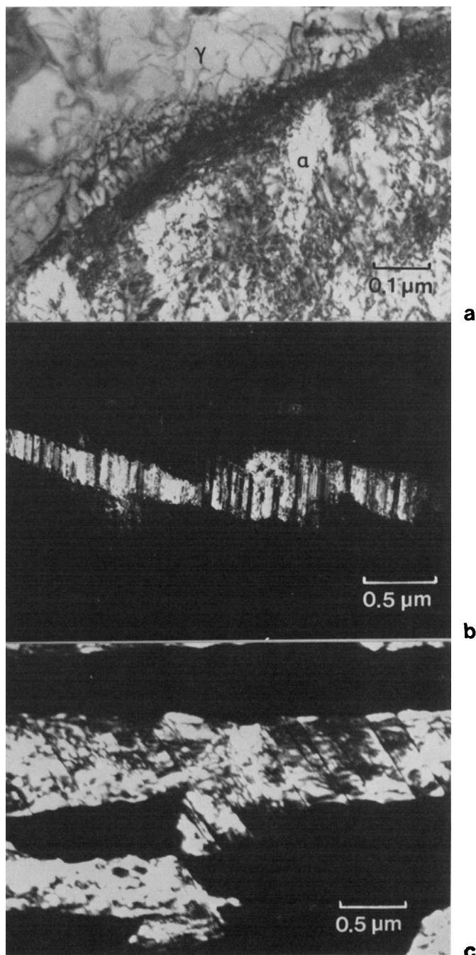
Fig. 7—Microstructural features of upper bainite formed after isothermal transformation at 350°C for 205 min. (a) Dislocation clusters associated with the bainitic ferrite/retained austenite interface. (b) Dark field image of upper bainitic retained austenite showing extensive faulting. (c) Dark field image of upper bainitic retained austenite showing accommodation slip steps.
