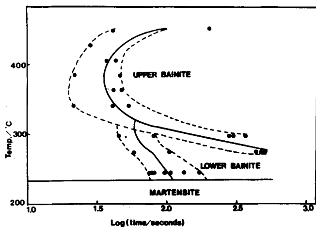
Fig. 1—Dilatometrically determined 5 pct transformation TTT curve.
