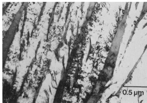
Fig. 6—Upper bainite formed after isothermal transformation at 350°C for 205 min. The retained austenite is the grey phase.
