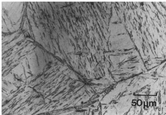
Fig. 5—Lower bainite formed after isothermal transformation at 246°C for 30 min.
