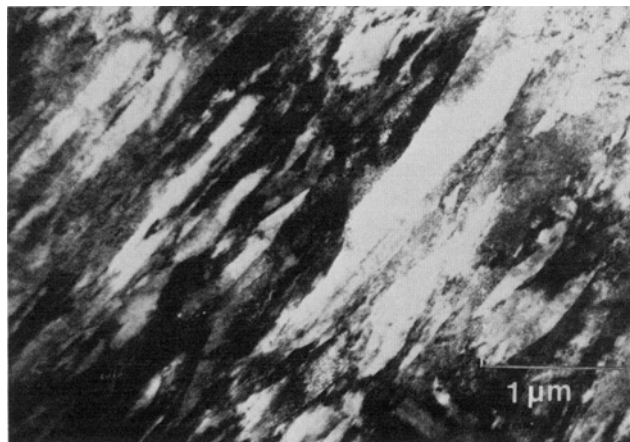
Fig. 11—Typical microstructure of lath martensite resulting from a direct quench following austenitization.
