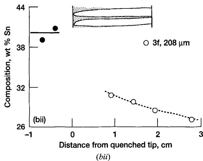
Fig. 5—Effect of primary dendrite spacings on the longitudinal macrosegregation for nearly constant mushy zone lengths (specimen 3d: C_0 = 27.0 at. pct Sn, H_f = 1.51 cm; specimen 3b: C_0 = 23.7 at. pct Sn, H_f = 1.45 cm; specimen 3c: C_0 = 23.4 at. pct Sn, H_f = 1.28 cm; specimen 3f: C_0 = 30.3 at. pct Sn, H_f = 1.90 cm; and specimen 3g: C_0 = 27.1 at. pct Sn, H_f = 1.89 cm). The primary dendrite spacings are indicated in the figures. (a) Macrosegregation along the length of the directionally solidified specimens. (b) Macrosegregation profiles within the quenched mushy zone (open symbols). Filled symbols indicate the composition of the melt at the time of quench. The mushy zones at the time of quench are indicated schematically. (i) specimen 3d ( \lambda_1 = 155 \mu\text{m} ) and (ii) specimen 3f ( \lambda_1 = 208 \mu\text{m} ).
