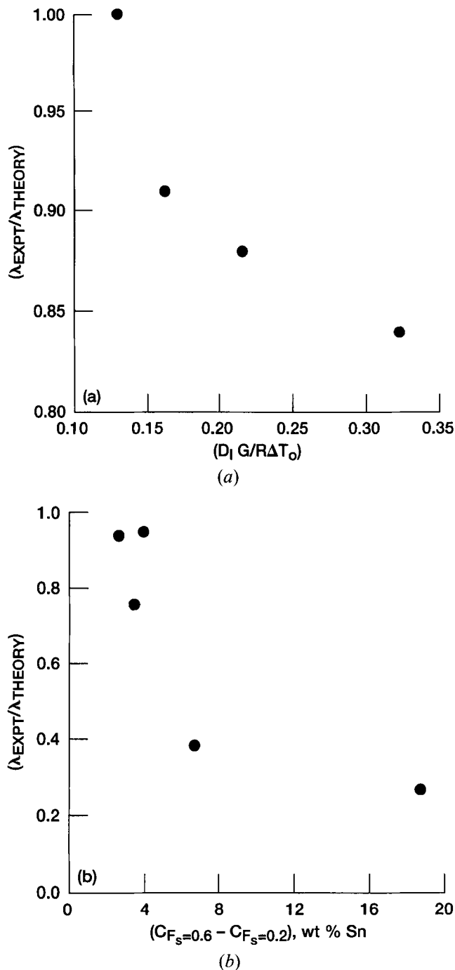
Fig. 7—Influence of convection on the primary dendrite spacings. (a) Ratio of the experimentally observed and theoretically predicted primary dendrite spacing vs D_l G/R\Delta T_0 . (b) Ratio of the experimentally observed and theoretically predicted primary dendrite spacing vs extent of macrosegregation ( C_{FS=0.6} - C_{FS=0.2} ).
