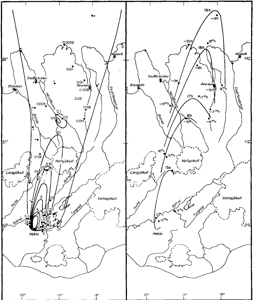
FIG. 15 — (a) Isopach map of the 1980 Hekla tephra fresh fallen. The volume of the tephra is given in Table 1. (b) Timing of the onset of the tephra fall on August 17th 1980.
