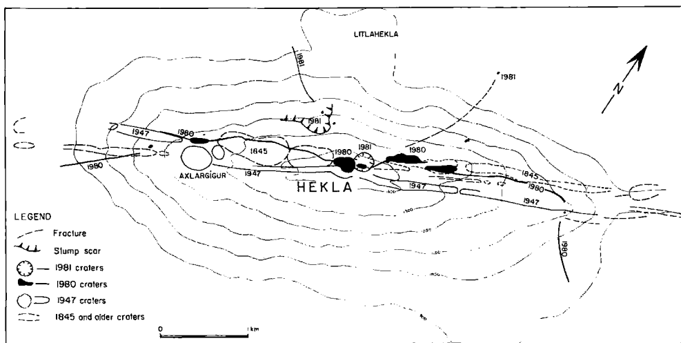
FIG. 18 — The distribution of craters and eruption fissures along the Hekla main ridge.
