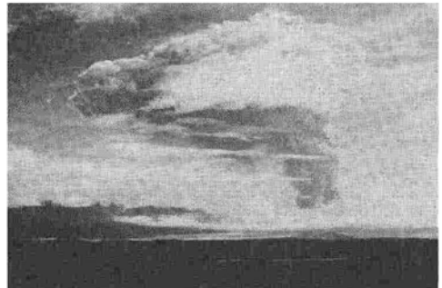
FIGS. 8-11 — Four photographs from a sequence taken from Uthlid in Biskupstungur 48 km NW of Hekla. The first one is taken at about 13:29 and the last one at about 13:36. Photo Sigurdur Hjaltason.
