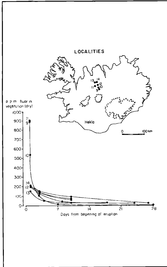
FIG. 17 — Variation of fluorine content of grass (ppm of dry matter) with time at some places in North Iceland. Numbers in circles refer to locations on the map. From FRIDRIKSSON (1981).
