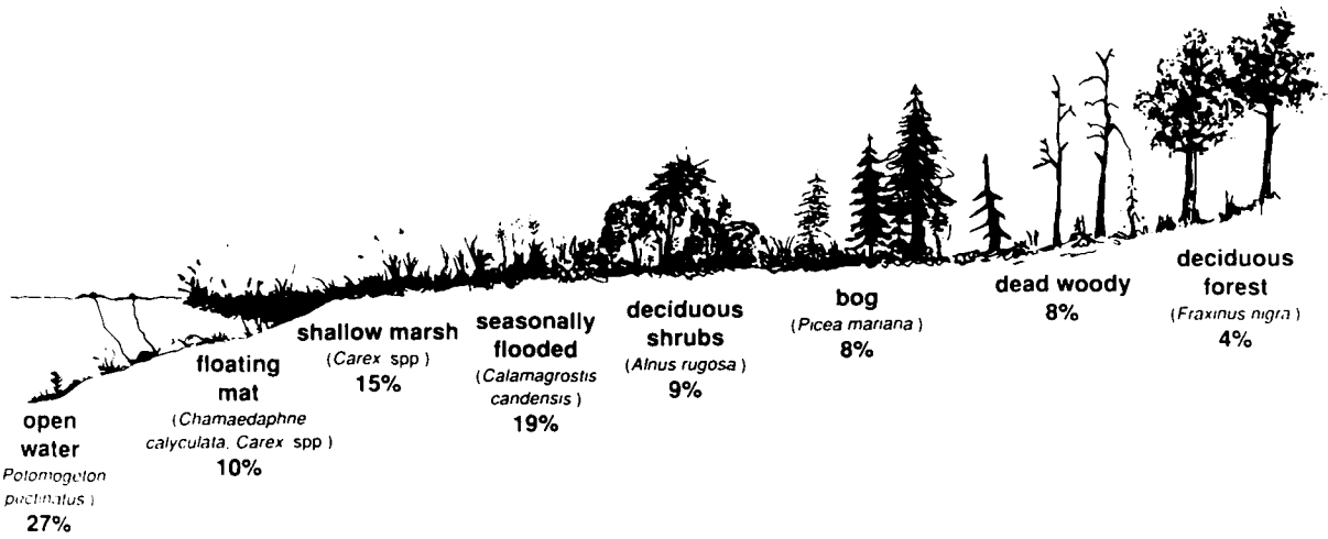
Fig. 2. Proportion of beaver impoundments in major vegetation types, 1986. Representative species shown in parentheses. 'Floating mat' includes floating meadow and floating woody mat. 'Bog' includes saturated and flooded bog. 'Deciduous forest' includes flooded deciduous and saturated deciduous forest.
