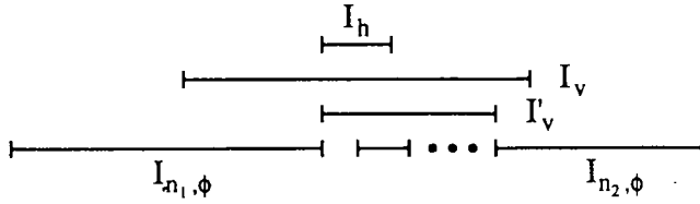
Figure 11. Bounding the length of I'_v .
