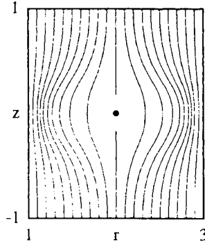
Figure 5. Contours of f .
