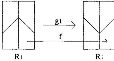
Figure 8. The map g_1 .
