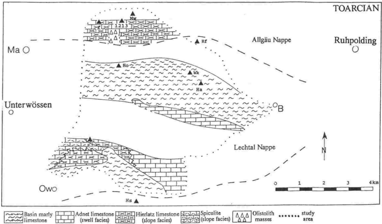
Fig. 10. Facies map of Upper Liassic basin and swell facies (Lechtal Nappe and southern Allgäu Nappe). During the Toarcian, a southern basin with marly limestones and an adjacent swell covered with condensed nodular limestones of Adnet facies is seen in the southern and middle Lechtal Nappe. Towards the west this swell seems to slope down as evidenced by a spiculite facies and resedimented echinoderm-rich Hierlatz limestones. Northward the swell transits into a basin with marly limestone deposition. Further northward across the nappe boundary into the Allgäu Nappe, a second swell is exposed. (Ma= Marquartstein, Uw= Unterwössen, Ow= Oberwössen, B= Brand, Ru= Ruhpolding; Ha= Haar-Alm, Hf= Hochfelln, Ho= Hochgern, Hs= Hochscharten, K= Kobelwand, Mw= Mehrentaler Wand, R= Rechenberg, Wk= Weißgrabenkopf) Facies patterns are displayed in the present-day tectonic constellation.
