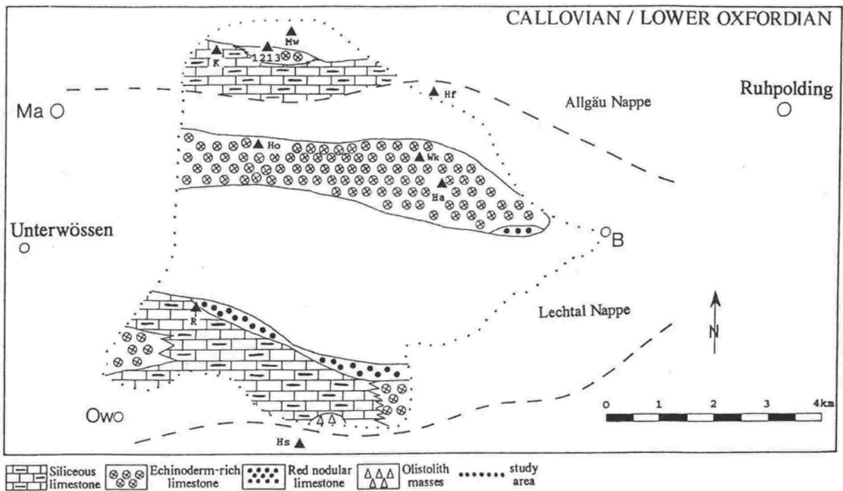
Fig. 11. Facies map of Upper Dogger to Lower Malm basin and swell facies (Lechtal Nappe and southern Allgäu Nappe). The Callovian/Lower Oxfordian configuration shows a broad swell covered with thick echinoderm-rich limestone units in the central Lechtal Nappe. Red nodular limestone deposited on the swellslope at its southeastern margin and in the southern Lechtal Nappe bear evidence of downslope mass movements (e.g. intraformational reworking). South and north of the swell siliceous limestones were infilled into basins. Furthermore, the southern basin shows outcrops of echinoderm-rich limestone facies at the western and eastern boundary of the area investigated. This may indicate downslope injections of echinoderm-rich sediments from nearby swells. Intensive downslope mass wasting is documented by an olistolith mass of siliceous limestones in the southern Lechtal Nappe. (for abbreviations see Fig.10)
