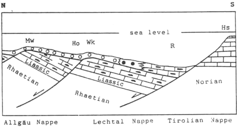
CALLOVIAN / LOWER OXFORDIAN
