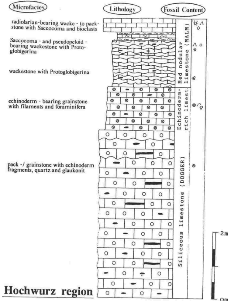
Fig. 7. Dogger and Malm series of the southern Allgäu Nappe (Hochwurz region): Basin facies with Dogger siliceous limestones dominate the lower part of the profile. Echinoderm-rich limestones were deposited during the Upper Dogger. The Malmian lithologies consists of red nodular limestones.
