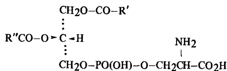
A phosphonolipid
