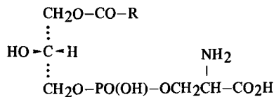
A 2-lysophospholipid
