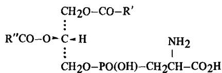
A phosphonolipid
