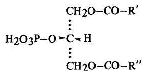
2-Phosphatidic acid
