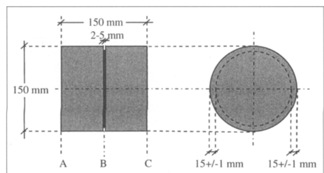
Fig. 1 – The geometry of the standard test specimen for uni-axial tensile testing. Planes A, B and C are parallel. Plane B is a symmetry plane. The total nominal length of the prepared specimen is 150 mm and the nominal diameter of the specimen is 150 mm. A central, circumferential notch with a depth of 15 mm +/- 1 mm is cut with a diamond saw. The resulting, maximum width of the notch is 2-5 mm.
