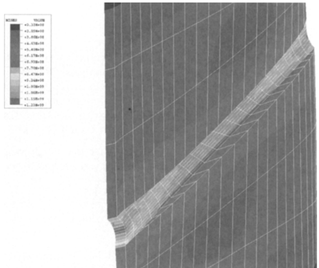
Fig. 5—Calculated (Mises) equivalent stress for the strain levels of Fig. 4, in the local gage coordinate system. Note the uniformity of the stress in the section gage. Most of the gage experiences stress levels in the range of 924–1000 MPa in this case.
