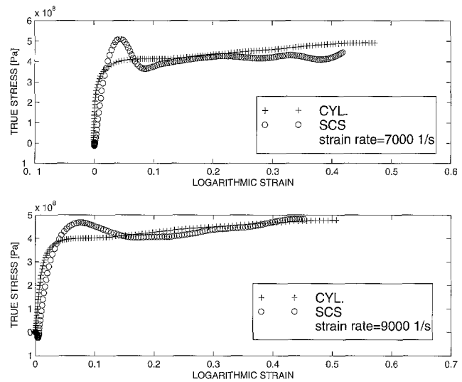
Fig. 10—Experimental results showing the comparison of the dynamic stress–strain curve of OFHC copper, obtained using compressed cylinders and SCS at strain rates of 7000 \text{ s}^{-1} and 9000 \text{ s}^{-1} respectively.
