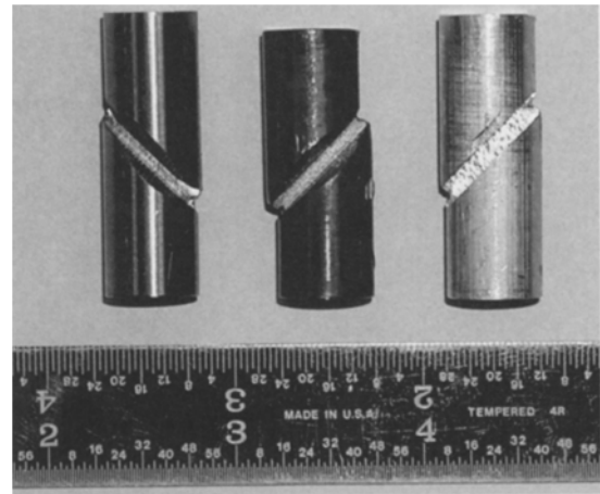
Fig. 2—Photographs of deformed specimens. From left to right: annealed Ti-6Al-4V titanium alloy, commercial OFHC copper and 6061-T351 aluminum alloy. The shear dominated deformation of the gage section is noticeable.
