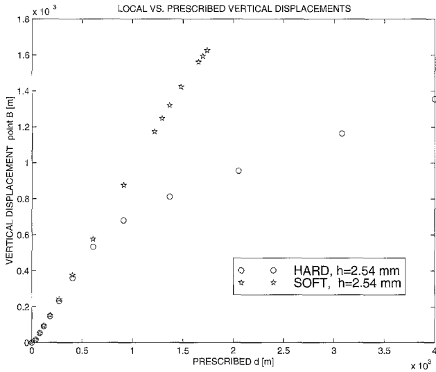
Fig. 3—Computed displacements of a representative point on the gage section, as a function of the prescribed vertical displacement. Note that for the “soft” material, there is a one to one correlation between these two factors, indicating that the cylindrical sections of the SCS do not alter the specimen stiffness.
