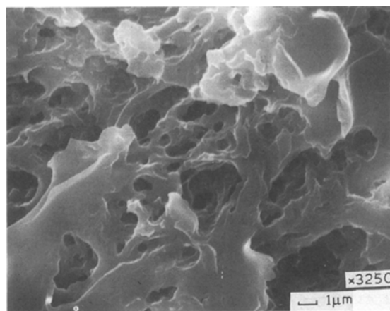
Figure 21 Fracture surface of uncrosslinked 10% rubber-modified phenoxy
