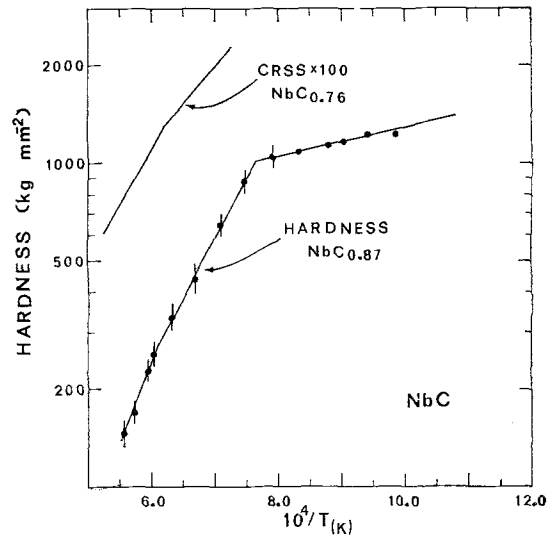
Figure 5 Log hardness versus inverse temperature for NbC. CRSS results are presented for comparison [3].
