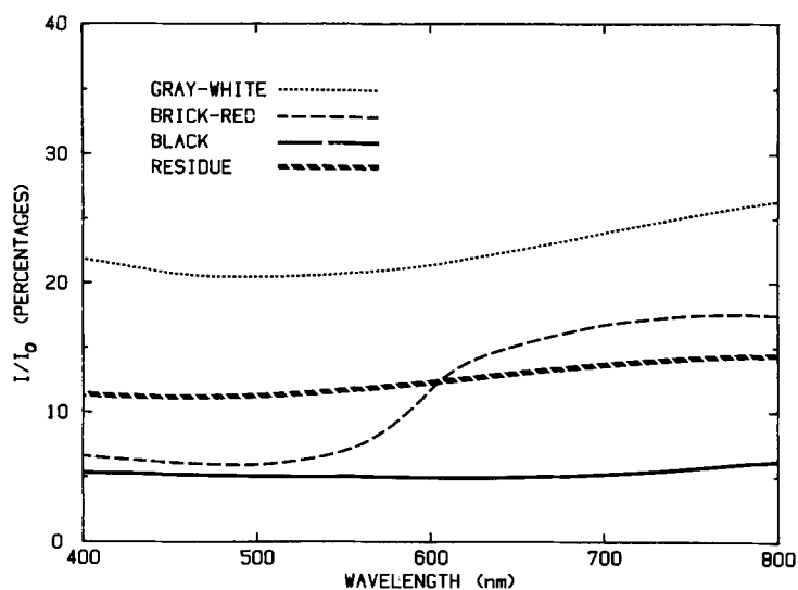
Fig. 1. Spectral distributions of reflected light 10 cm above a wheat residue-cover and dry gray-white, brick-red and black soils relative to direct sunlight (which was considered to be 100% for each measured wavelength).
