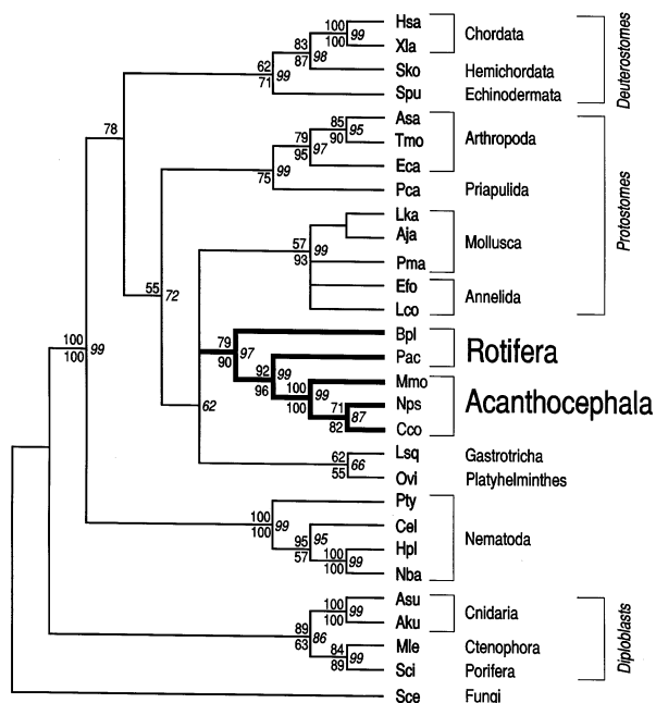
Fig. 1. The tree is a consensus derived from neighbor-joining, maximum parsimony, and maximum likelihood analyses of a secondary structure based alignment of near-complete 18S rRNA genes from 29 taxa. Numbers above and below each fork represent percentage of 1,000 bootstrap replicates that support the branch in the maximum parsimony tree and the neighbor-joining tree, respectively, and are shown only where greater than 50%. Numbers to the right of each branch are confidence-probability values that the branch length is significantly greater than zero and are shown only when greater than 50. See text for the definitions of the three-letter codes at each terminal node.
