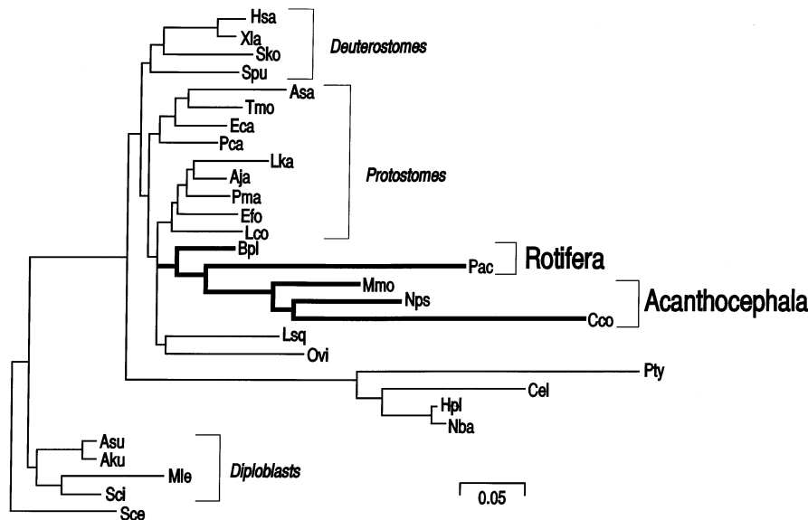
Fig. 2. Neighbor-joining tree from Fig. 1 showing branch lengths drawn to scale (number of substitutions per site). See Fig. 1 for bootstrap and confidence-probability values. Phylum names other than Acanthocephala and Rotifera are omitted for clarity. Removal of sequences representing the taxa Pac or both Pac and Coo from the analysis did not change the topology of the tree.
