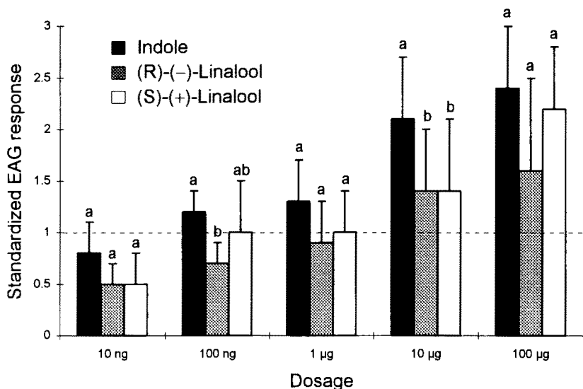
FIG. 2. EAG dose responses of female medfly antennae to selected known volatile compounds released by calling males. Stimuli were commercial or synthetic standards. Standard deviations of mean responses are presented as error bars. Dotted line indicates the mean response to the hexanol standard (10 \mu\text{g} ). Dosage means with the same letter are not significantly different by Student's t test at P < 0.05 ( N = 9 ).
