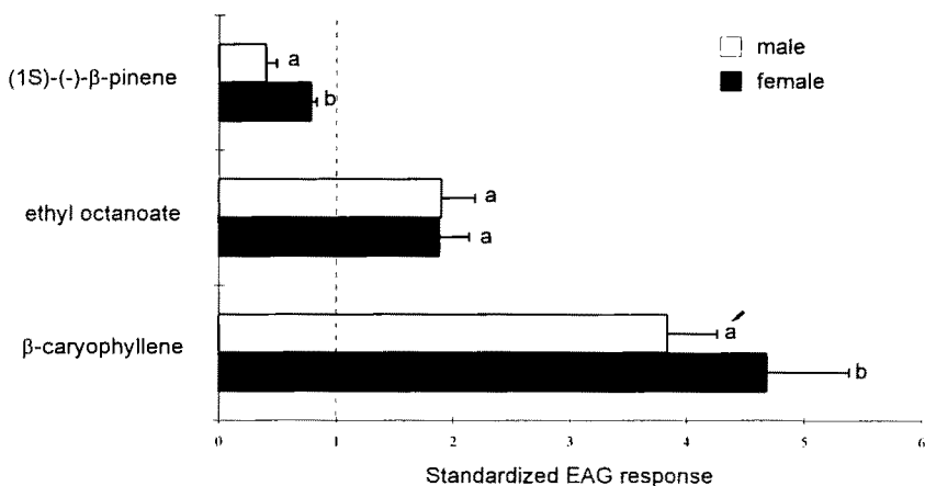
FIG. 6. EAG responses of male and female medfly antennae to commercial or synthetic compounds (100 ng) identified from ripe mango. Standard deviations of mean responses are presented as error bars. Dotted line indicates the mean response to the hexanol standard (10 \mu g). Male and female response means from the same compound with the same letter are not significantly different by Student's t test at P < 0.05 ( N = 10 ).
