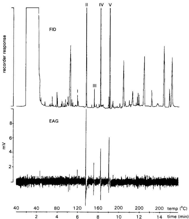
FIG. 1. Reconstructed simultaneously recorded gas chromatogram [flame ionization detector (FID)] of trapped volatiles of calling male medflies (top) and electroantennogram (EAG) of a female medfly antenna (bottom). EAG active compounds are labeled I, II, III, IV, and V (see text for details).
