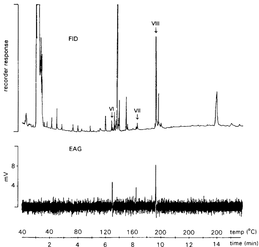
FIG. 3. Reconstructed simultaneously recorded gas chromatogram [flame ionization detector (FID)] of trapped volatiles of ripe mango (top) and electroantennogram (EAG) of a female medfly antenna (bottom). EAG active compounds are labeled VI, VII, and VIII (see text for details).
