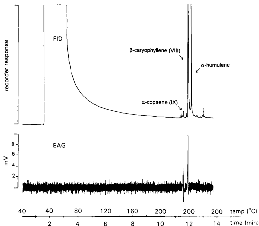
FIG. 5. Reconstructed simultaneously recorded gas chromatogram [flame ionization detector (FID)] of a mixture of \alpha -copaene, \beta -caryophyllene, and \alpha -humulene (top) and electroantennogram (EAG) of a female medfly antenna (bottom). EAG active compounds are labeled VIII and IX (see text for details).
