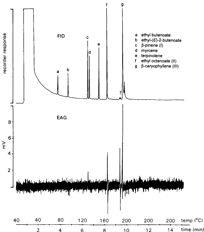
FIG. 4. Reconstructed simultaneously recorded gas chromatogram [flame ionization detector (FID)] of a mixture of commercial and synthetic compounds identified from ripe mango (top) and electroantennogram (EAG) of a female medfly antenna (bottom). EAG active compounds are labeled VI, VII, VIII, and ? (see text for details).
